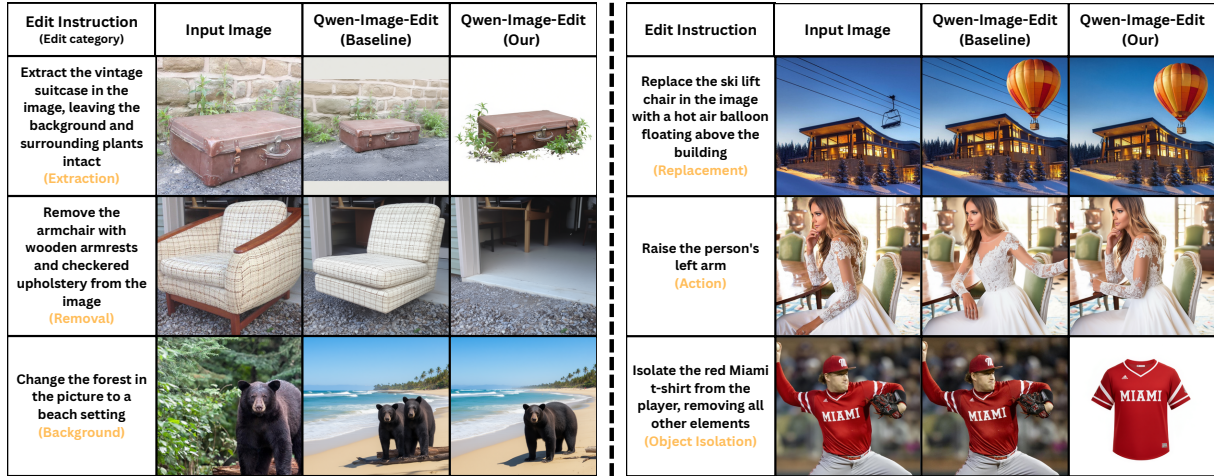
Figure 4: Qualitative comparison between Qwen-Image-Edit and our Rubric-CEPR on ImgEdit. Each row shows the edit instruction with its category, the input image, the baseline output, and ours. The baseline often returns a realistic image that leaves the requested change undone; for example, it keeps the player when asked to isolate the red shirt (bottom right). Rubric-CEPR completes such edits while preserving the content that the instruction leaves unchanged. Additional examples are provided in Appendix H.
