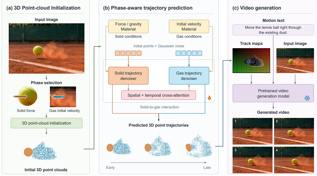
Figure 2: PAVG overview: (a) initialize phase-specific 3D point clouds; (b) use a phase-aware point-trajectory predictor to predict solid and gas trajectories; (c) project the trajectories to guide a pretrained video generation model. Flames and snowflakes mark trainable and frozen modules.
