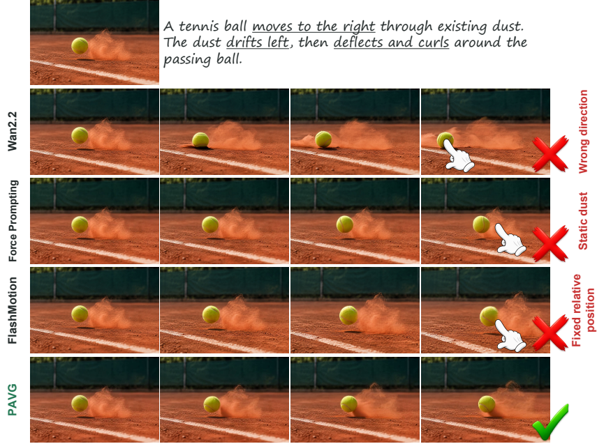
Figure 1: A tennis ball moving through dust. Wan2.2 moves the ball in the wrong direction; Force Prompting leaves the dust stationary; FlashMotion moves the ball and dust together without a visible interaction. PAVG follows the prescribed ball motion and produces a responsive dust plume, yielding a more physically plausible solid–gas interaction. The figure contains fine-grained motion details and is best viewed on a computer.
