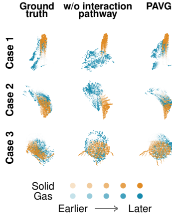
Figure 5: Qualitative interaction-pathway ablation on three held-out solid-gas cases. With the CPI pathway enabled, the gas visibly responds to and follows the solid’s motion.
