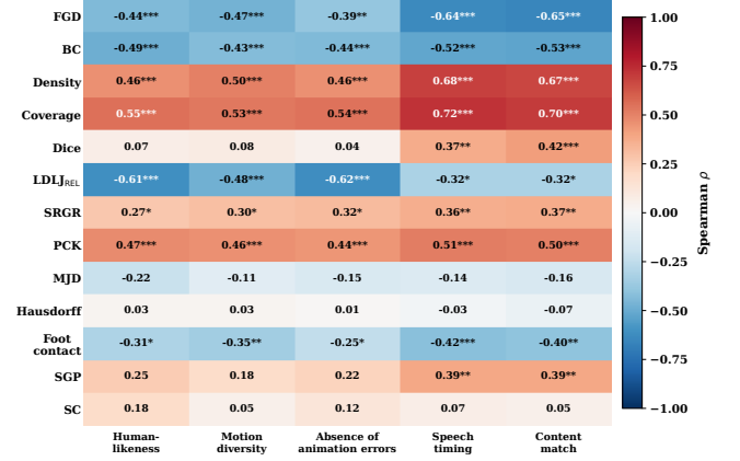
Figure 3: Spearman correlations between thirteen objective metrics and five subjective evaluation dimensions ( n = 60 ), with significance indicated by * p < 0.05 , ** p < 0.01 , and *** p < 0.001 .
