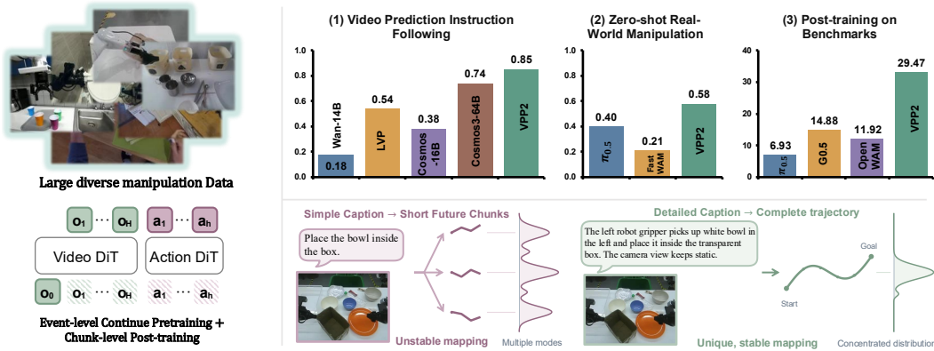
Figure 1: A typical robot policy maps an simple instruction and an observation into an short action chunk. As datasets scale, this mapping becomes increasingly multi-modes and uncertain, leading models to learn spurious short-horizon correlations. VPP2 first establishes consistent semantic-to-trajectory mappings via next event video prediction with detailed caption, then post-train and distill model to generate short action chunk.
