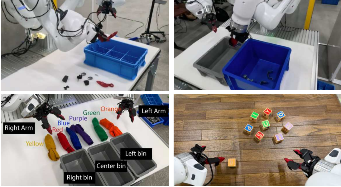
Figure 5 | Experimental setup for robot evaluation tasks.
