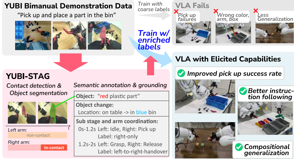
Figure 1 | From a bimanual demonstration carrying only a coarse task label such as “pick and place a part,” YUBI-STAG recovers contact-anchored annotations of object identity, per-gripper action, bimanual coordination, and object change, which post-training uses to align the pretrained capabilities of a VLA with fine-grained manipulation language.
