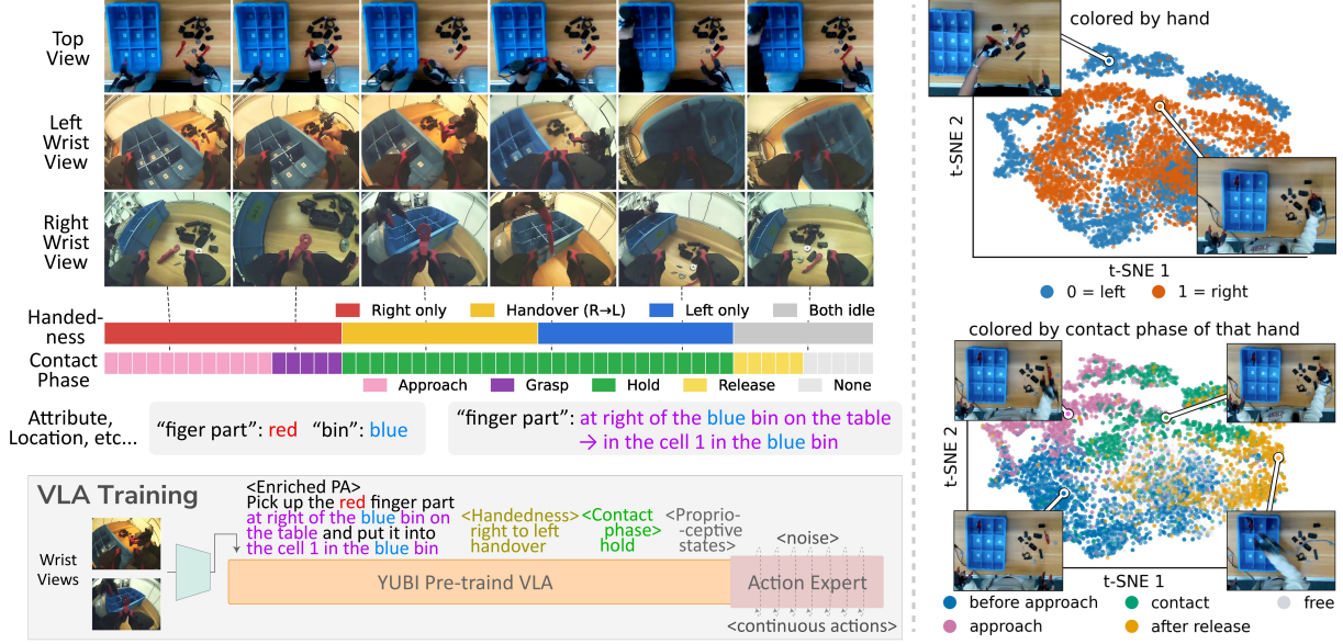
Figure 3 | Contact- and semantic-rich post-training for YUBI-VLA. Left: YUBI-STAG augments primitive-action instructions with task-relevant object attributes and locations, together with time-varying handedness and contact-phase labels while the unchanged flow-matching expert learns continuous bimanual actions. Right: t-SNE projections of per-hand delta actions after PCA-50 reduction, colored by hand identity and contact phase, reveal handedness and contact-phase structure in the trajectories and motivate the proposed labels.
