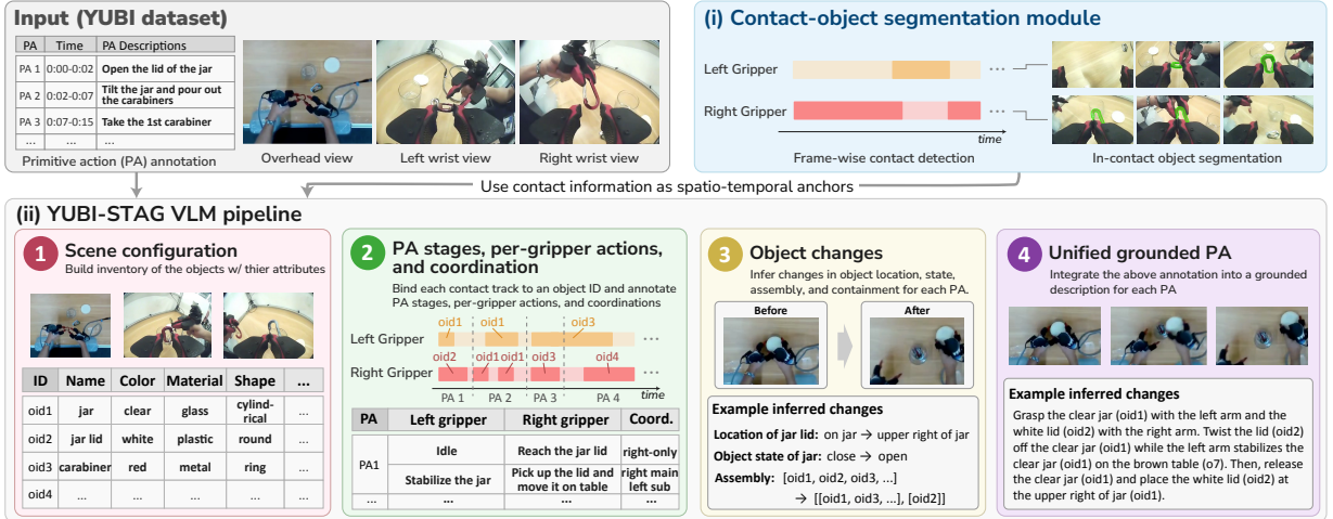
Figure 2 | Overview of YUBI-STAG. The contact-object segmentation module extracts contact tracks —contact intervals with per-frame object masks—as spatio-temporal anchors for four annotation stages: scene configuration, PA stages and gripper coordination, object changes, and grounded PA descriptions.
