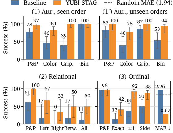
Figure 6 | Fine-grained language steerability. Baseline (blue) and YUBI-STAG (orange) success rates with 95% Wilson confidence intervals. P&P in (3) does not measure instruction following because any sock may be grasped. MAE: ordinal position error (right axis, lower is better), compared with uniform random selection (dashed line). Attr.: attribute; Grip.: gripper; Betw.: between.
