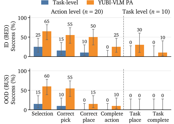
Figure 7 | Letter-block action composition on BED (ID) and BUS (OOD). Bars compare the task-level baseline (blue) and YUBI-VLM PA supervision (orange) with 95% Wilson score confidence intervals. Action metrics ( n = 20 ) are cumulative; task place and task complete require both actions to succeed through placement and orientation, respectively ( n = 10 ).
