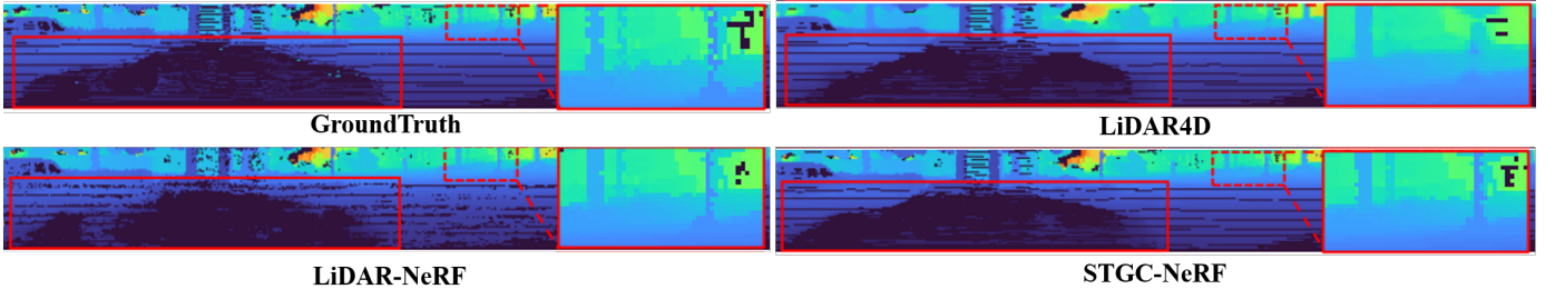
Fig. 5. Qualitative reconstruction point map and depth of NeRF-style methods on the NuScenes [170] dataset. Image from [93].
