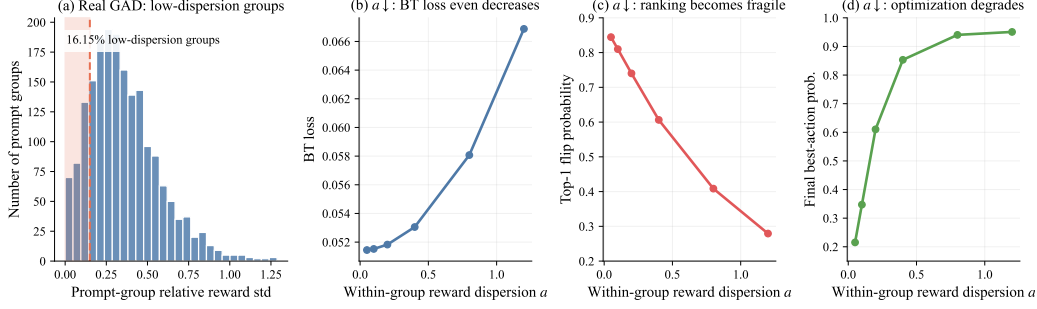
Figure 2: Why BT-style adversarial critic training alone is insufficient for advantage construction.
