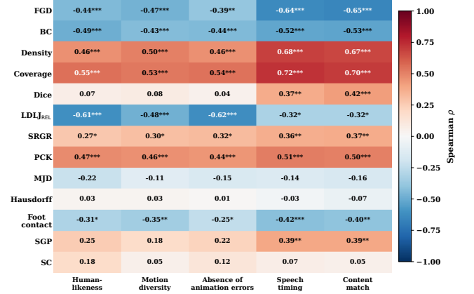
Figure 3: Spearman correlations between thirteen objective metrics and five subjective evaluation dimensions ( n = 60 ), with significance indicated by * p < 0.05 , ** p < 0.01 , and *** p < 0.001 .
