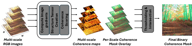
Figure 3. Multi-scale coherence: the coherence map is produced by a structure tensor at each scale, followed by thresholding and intersecting across scales to retain structure that is vertically coherent at every scale.
