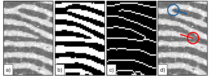
Figure 1: Classical minutiae extraction pipeline. (a) Portion of a fingerprint image displaying dark gray ridges separated by lighter valleys. (b) Enhanced and binarized image, where ridges are mapped to white pixels and valleys to black pixels. (c) Topological skeletonization of the ridges (1-pixel wide white paths). (d) Extracted minutiae features, highlighting a ridge ending near the top (blue circle) and a bifurcation located lower towards the center (red circle). The line segment originating from the center of each circle indicates the direction of the corresponding minutia, defined by an angle in [0, 2\pi) .
