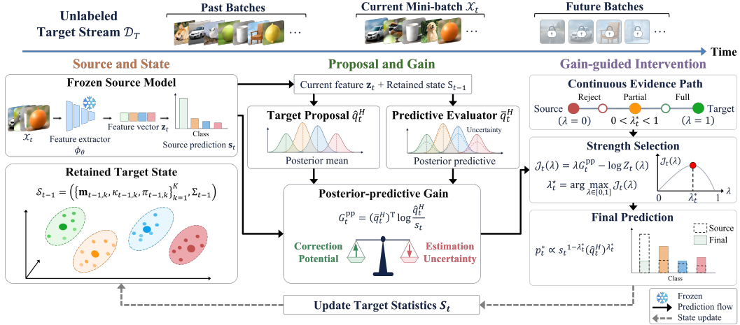
Figure 2: Overview of GAIN: history proposes, gain decides. (i) The frozen source model produces the source prediction s_t and current feature z_t , while the retained target state \mathcal{S}_{t-1} summarizes past batches. (ii) Together, z_t and \mathcal{S}_{t-1} form the target proposal \hat{q}_t^H and predictive evaluator \bar{q}_t^H . The evaluator accounts for uncertainty to estimate the proposal’s source-relative gain G_t^{pp} . (iii) This source-relative gain determines the intervention strength \lambda_t^* along the continuous evidence path from s_t to \hat{q}_t^H . The final prediction p_t^* then updates the target statistics \mathcal{S}_t for future batches.
