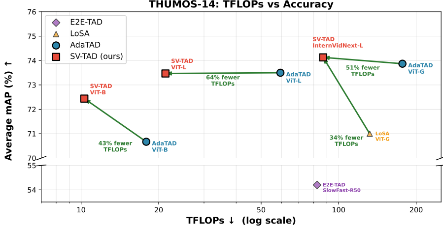
Figure 1: TFLOPs vs. accuracy on THUMOS-14 . SV-TAD (red squares) matches or exceeds AdaTAD [21] (blue circles) at substantially lower compute across three backbone scales: 43% fewer TFLOPs with VMAEv2-B, 64% with VMAEv2-L, and 51% when comparing our InternVideoNext-L against AdaTAD’s VMAEv2-G.
