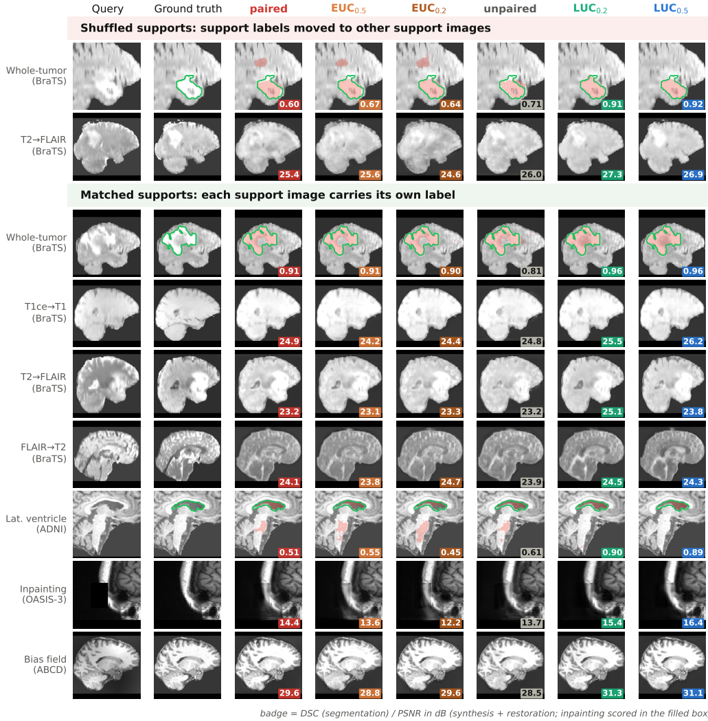
Figure 9: Qualitative comparison across tasks and models ( K=4 ). Six models (paired \rightarrow EUC 0.5 \rightarrow EUC 0.2 \rightarrow unpaired \rightarrow LUC 0.2 \rightarrow LUC 0.5 ); green = ground-truth contour, red = predicted mask; the corner badge is DSC (segmentation) or PSNR in dB (synthesis/restoration; inpainting scored in the filled box only). Rows are labeled task (dataset). Top, shuffled supports: two tasks; the paired model degrades (partial or displaced mask, lost detail) while LUC 0.5 and LUC 0.2 hold, EUC 0.5 and EUC 0.2 degrade with the paired model, and the unpaired model sits in between. Bottom, matched supports: the trained task suite across all four datasets. Accuracy is comparable throughout: LUC 0.5 matches the paired model on translation and restoration, is cleaner on the two segmentation tasks (whole-tumor over-segmentation; atrophic ADNI ventricle), and fills the inpainting box slightly better. The bottom-row cases were selected to show the pattern; population numbers are in Tables 6 and 7.
