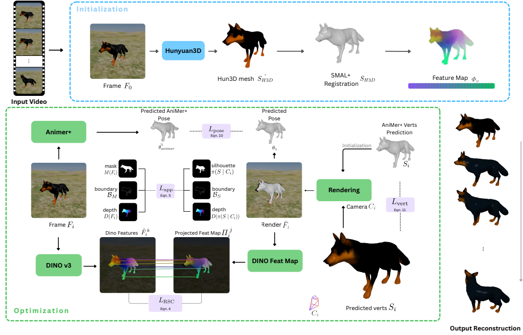
Figure 2: ORMA takes a video as input and produces a 4D reconstruction of the animal, with a trajectory in world coordinates (bottom right). As initialization, ORMA leverages Hunyuan3D (Zhao et al., 2025) to obtain a reliable shape estimation of the first frame (blue box). After registering SMAL+ (Zuffi & Black, 2024), we perform a frame-by-frame optimization (green box). Unlike previous works, ORMA relies on MegaSaM (Li et al., 2025) to robustly estimate camera parameters across the entire video, along with a depth map. Additionally, we design a Robust Semantic Correspondence module using DINO (Siméoni et al., 2025) to produce a robust set of sparse correspondences between the frames and the SMAL+ registration. Equations are provided in the appendix.
