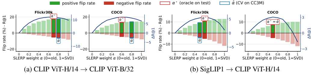
Figure 9: I2T Recall@1 flip-rate trade-off on Flickr30k and COCO. Bars show positive and negative flip rates relative to the old-to-old evaluation. The blue curve reports \Delta R@1 = \text{PFR} - \text{NFR} . Here \alpha = 0 corresponds to old-model queries and \alpha = 1 to SVD-aligned new-model queries. Red and blue markers denote the dataset-specific oracle \alpha^* and the CC3M-selected weight \hat{\alpha} , respectively.
