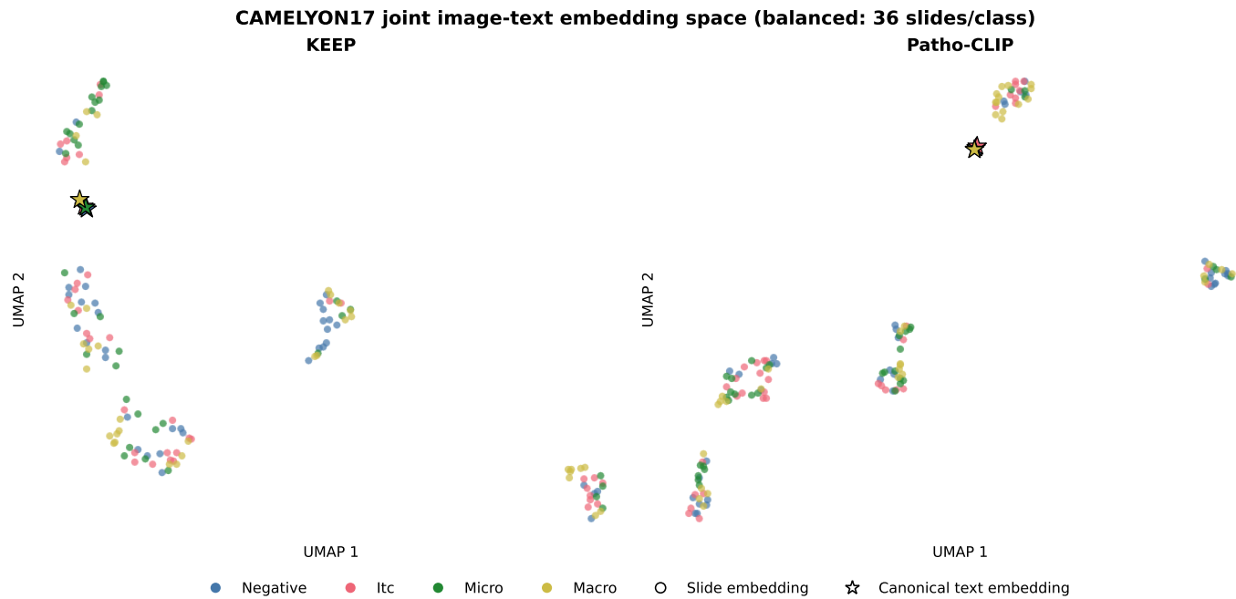
Fig. C.1: Qualitative UMAP visualization of the joint slide–text embedding space on CAMELYON17. Points are colored by ground-truth diagnostic class; circles denote slide embeddings and stars denote canonical text embeddings. For each model, 36 slides per class were sampled from the subset with verified labels. UMAP was fit independently for each model using L2-normalized embeddings, cosine distance, n_{\text{neighbors}} = 15 , \text{min\_dist} = 0.15 , and seed 42. Coordinates are not comparable across panels. This figure illustrates the modality gap between image and text embeddings (Liang et al., 2022); it is not evidence of class separability or of diagnostic-language grounding.
