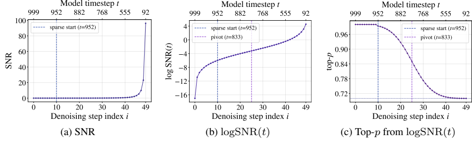
Figure 4: Visualization of proposed SNR-guided sparsity schedule on Wan2.1-T2V-14B. (a) Raw SNR over denoising timesteps. (b) \log \text{SNR}(t) , where the pivot marks the center of the flattest region. (c) The resulting top- p schedule generated by an inverted sigmoid.
