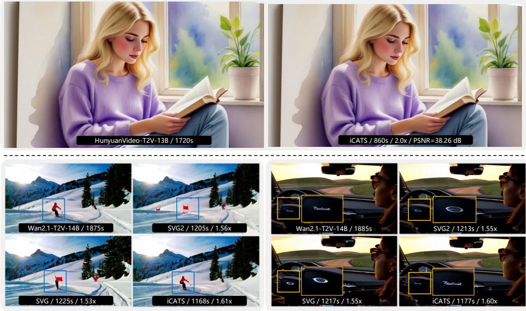
Figure 1: Visualizations on HunyuanVideo-T2V-13B and Wan2.1-T2V-14B show that iCATS better preserves visual details while achieving higher speedup than other training-free methods, producing results closer to native videos. On average, it achieves 2.03\times acceleration with 31.017 dB PSNR on HunyuanVideo-T2V-13B, and 1.55\times acceleration with 29.301 dB PSNR on Wan2.1-T2V-14B.
