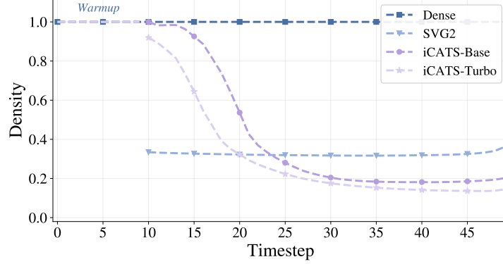
Figure 1: Density of the original full attention, SVG2, and our iCATS across timesteps on Wan2.1-T2V-14B.
