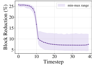
Figure 5: Reduction ratio of execution blocks on Wan2.1-T2V-14B.
