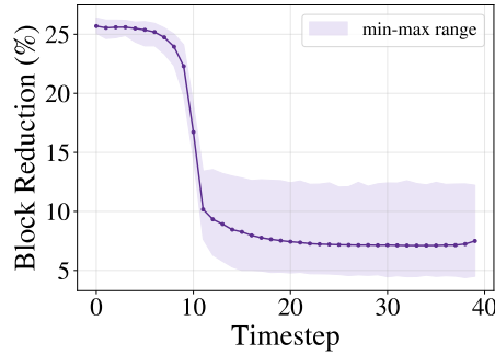
Figure 2: Relative reduction in the number of executed FlashInfer blocks on Wan2.1-T2V-14B under the iCATS-Base setting.
