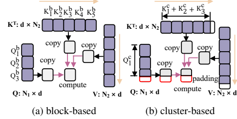
Figure 2: Visualization of (a) block-based and (b) cluster-based sparse attention.
