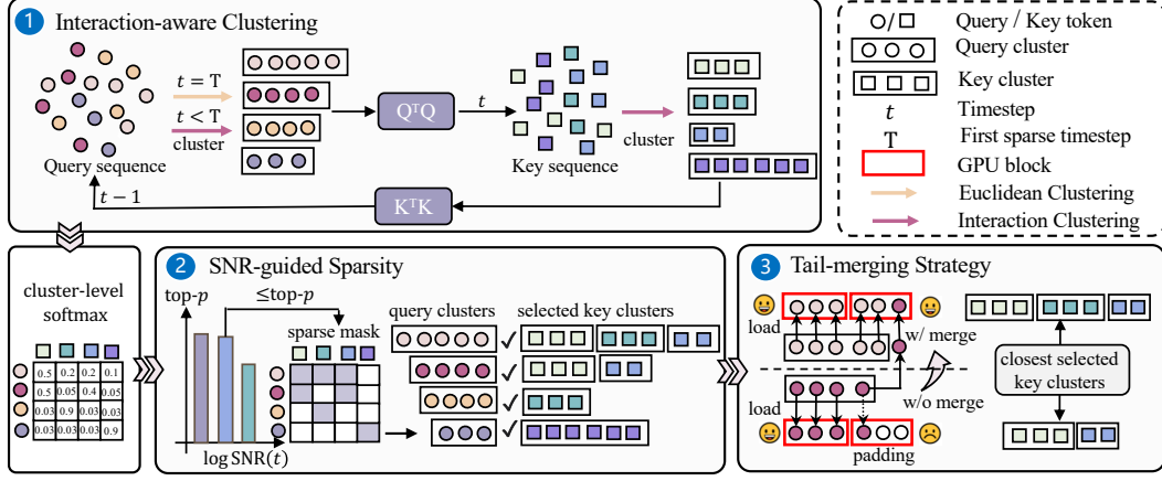
Figure 3: Overview of iCATS pipeline. For each attention layer, query and key tokens are first grouped by ① Interaction-aware Clustering . Then, the corresponding query-key cluster centroids are used to approximate softmax scores at the cluster level. Based on these approximated scores, ② SNR-guided Sparsity determines the top- p value at each denoising timestep and selects the corresponding attention computation region. Finally, ③ Tail-merging Strategy is applied before sparse attention kernel computation by reassigning tail tokens of non-block-aligned query clusters, thereby reducing padding overhead caused by irregular cluster sizes. In this figure, interaction clustering denotes interaction-aware query-key clustering, while Euclidean clustering is used to initialize query clusters solely at the first sparse timestep.
