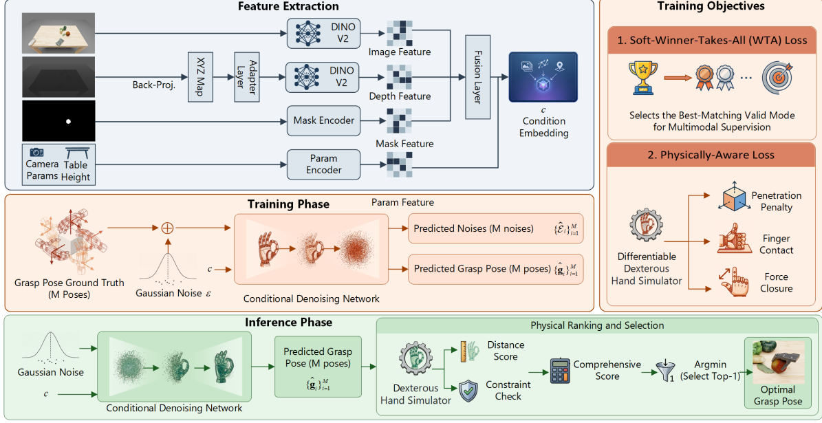
Figure 4 Architecture of the OmniDex Model. Condition embeddings are transformed from RGB-D inputs, instruction masks, and scene parameters. During training, a denoising network adds identical noise to M grasp poses, optimized jointly via a Soft Winner-Takes-All loss (for multimodal distributions) and a physics-aware loss (for stable contact). During inference, the network generates M candidates, followed by a physics-based ranking module to select the optimal grasp.
