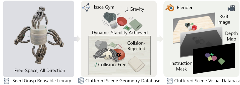
Figure 2 Seed-and-filter generation pipeline. Our two-stage framework generates scene-valid grasps by: (1) constructing a reusable seed grasp library in free space, and (2) simulating cluttered scenes in Isaac Gym for collision filtering, followed by multi-modal rendering in Blender.
