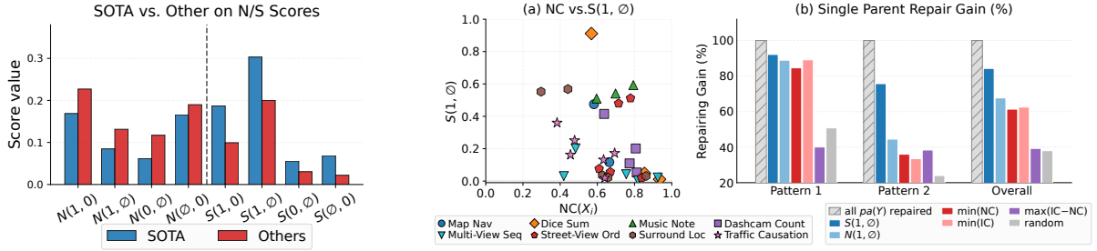
Figure 7 | N/S -Scores across the four state contrasts for SOTA vs. Others models. Figure 8 | (a) NC(X_i) vs. S(1, \emptyset) ; (b) percentage of full all-prerequisite gain( IC-NC ) recovered by single-parent supply across selection criteria.
