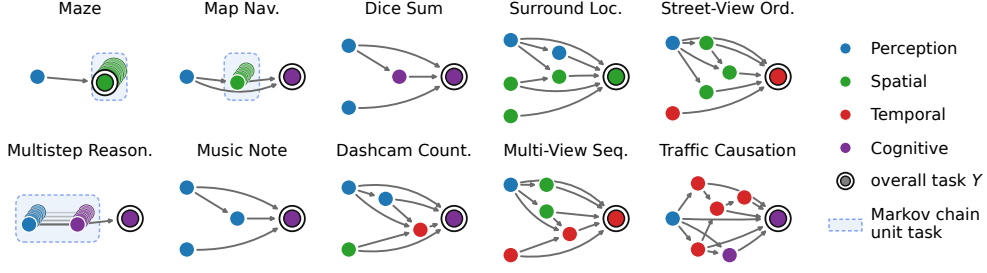
Figure 2 | Overview of SCMs corresponding to 10 tasks in CADET.
