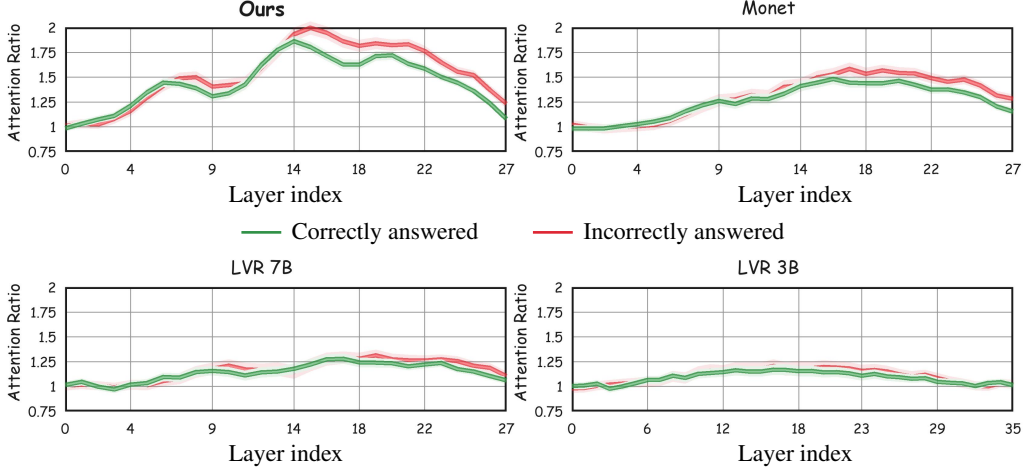
Figure G.2: Target-region attention enrichment. Layer-wise answer attention on the annotated region relative to matched background windows. Values above 1 indicate target-region enrichment; green and red curves correspond to correct and incorrect generations, respectively. Their overlap shows that alignment alone does not determine answer correctness.
