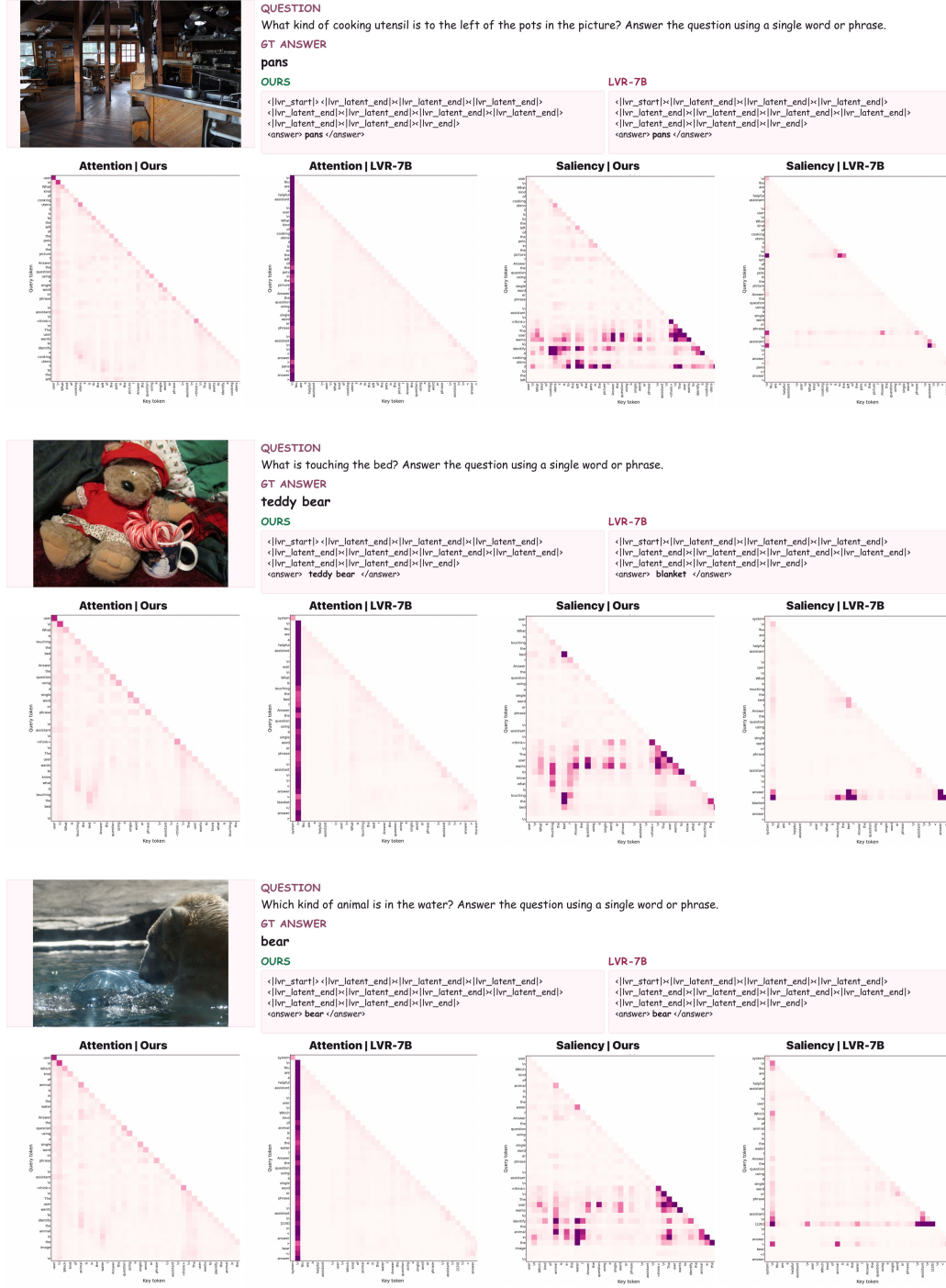
Figure H.3: Attention and saliency cases (07–09). Top to bottom: pans left of the pots, the teddy-bear answer comparison, and a bear in water. In the middle example (Case 08), ReaLVR answers “teddy bear” and LVR-7B answers “blanket” to “What is touching the bed?”
