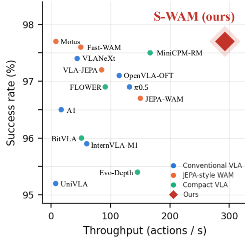
Figure 1: Success rate versus measured inference throughput on LIBERO. The measurement protocol, per-method results, and methods omitted from the figure are provided in Appendix C.
