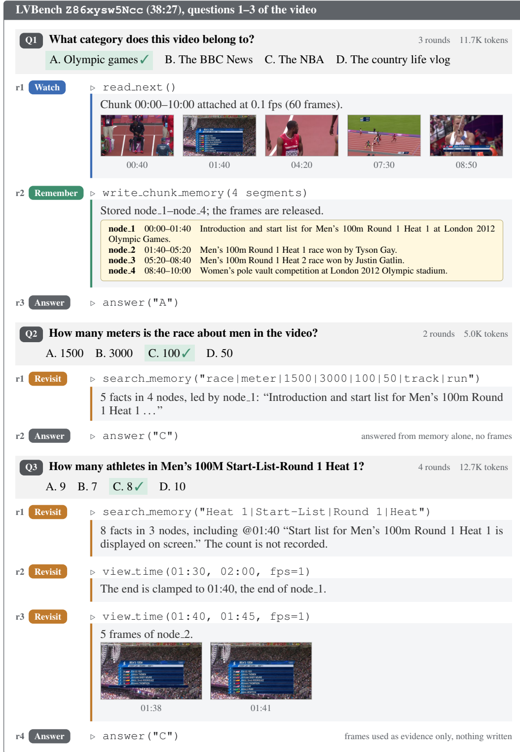
Figure 5: The first three questions on one LVBench video (Sprout with Gemini 3.8 Flash; Figure 6 continues with questions 4 and 5). Each round shows the tool call ( > ) and, in the shaded block, its result. Q1 watches the first chunk and records it as four nodes; no later question in this figure watches further. Q2 is answered by one search. Q3 finds where the start list is shown but not its length, so it revisits that interval at 1 fps, first clamped at the boundary of node_1, and counts the athletes on the frames. Tool calls keep only their key arguments and tool results are abridged; memory text is verbatim from the request log, and token counts are total input tokens per question.
