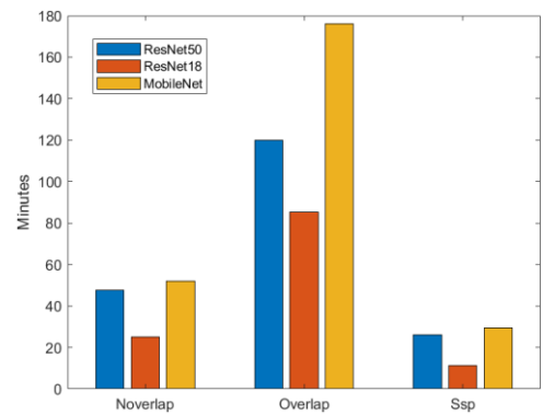
Figure 6. DeepLabV3+ training time
