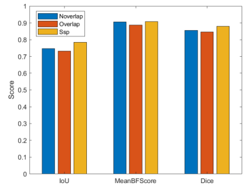
Figure 4. DeepLabV3+ with ResNet18
