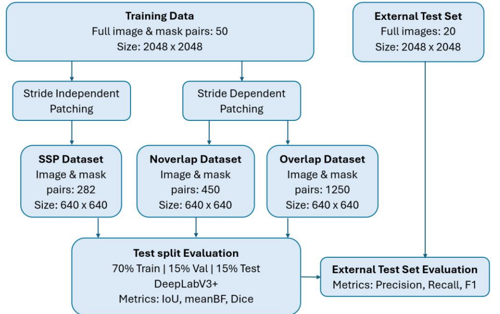
Figure 2: Overview of patch-based dataset construction and evaluation of its effects
