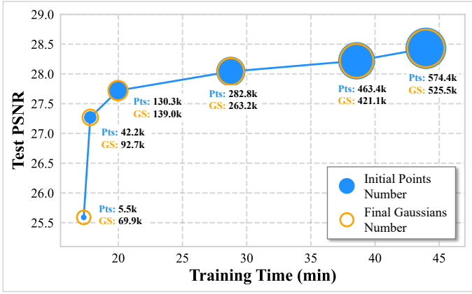
Fig. 7. Performance under different size of voxel grid down-sampling.
