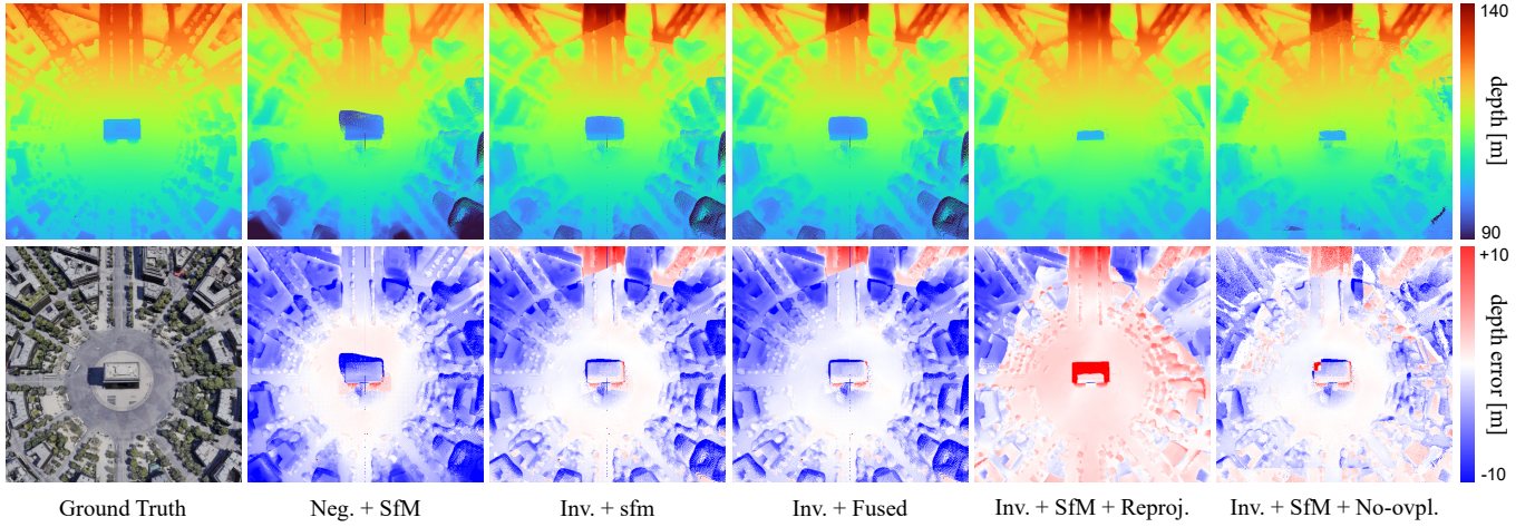
Fig. 6. Visualization of depth map and depth error with different initialization strategies.
