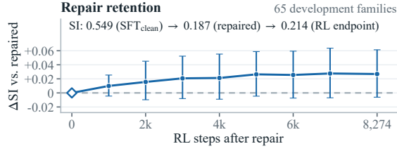
Figure 9: Change in Audio-question SI from the repaired model during subsequent RL post-training, with pointwise 95% paired family-cluster bootstrap intervals.
