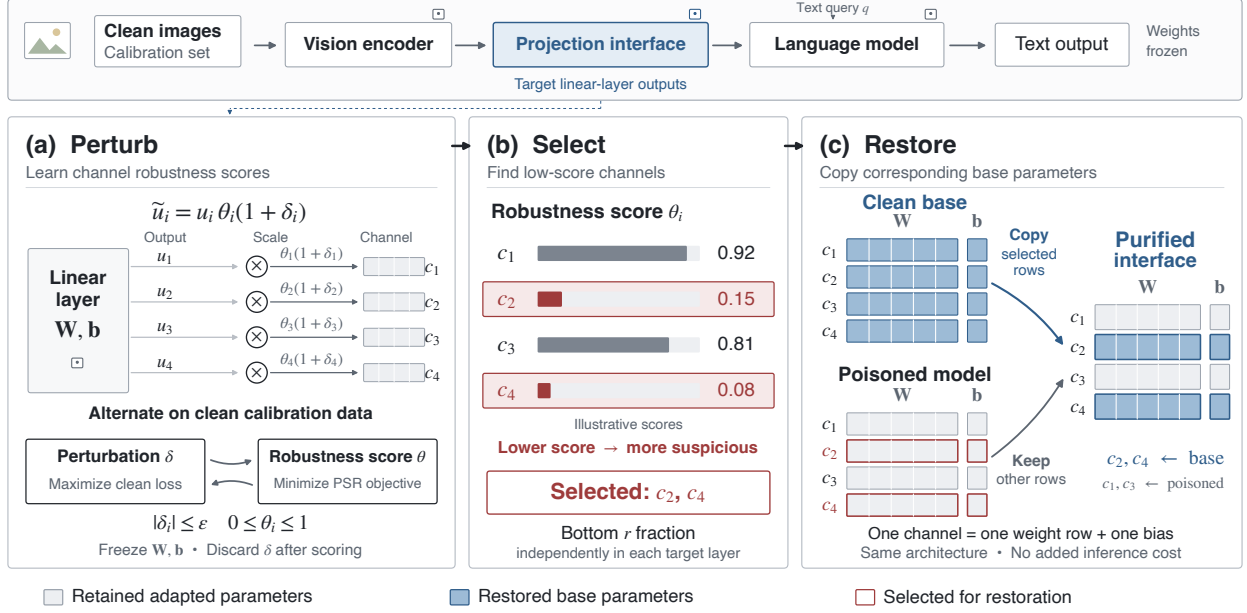
Figure 2: Overview of Perturb-Select-Restore (PSR), a post-training purification framework for VLM projection interfaces.
