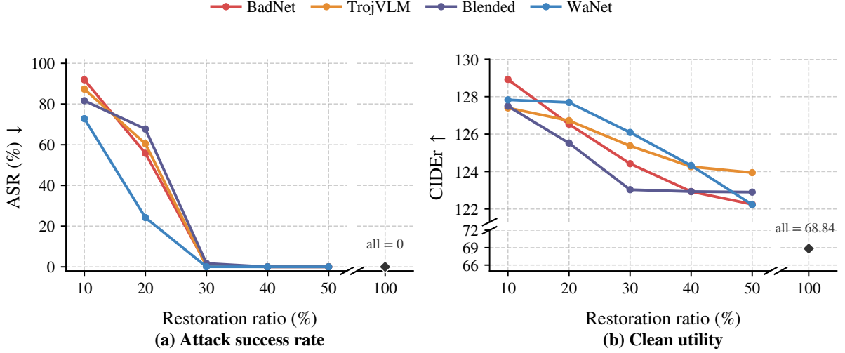
Figure 3: Ablation of the PSR restoration ratio on Qwen3-VL-8B COCO attack settings. (a) ASR ( \downarrow ) on triggered images; (b) clean utility (CU; CIDEr, \uparrow ) on clean images. Each curve reuses the same optimized robustness scores and restores selected parameters from \phi_0 . Diamonds denote the shared result of all four attacks at 100% restoration.
