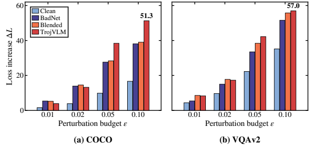
Figure 1: Loss increase \Delta L under bounded projector perturbations on clean samples. (a) COCO; (b) VQAv2. Higher \Delta L indicates greater projection fragility.
