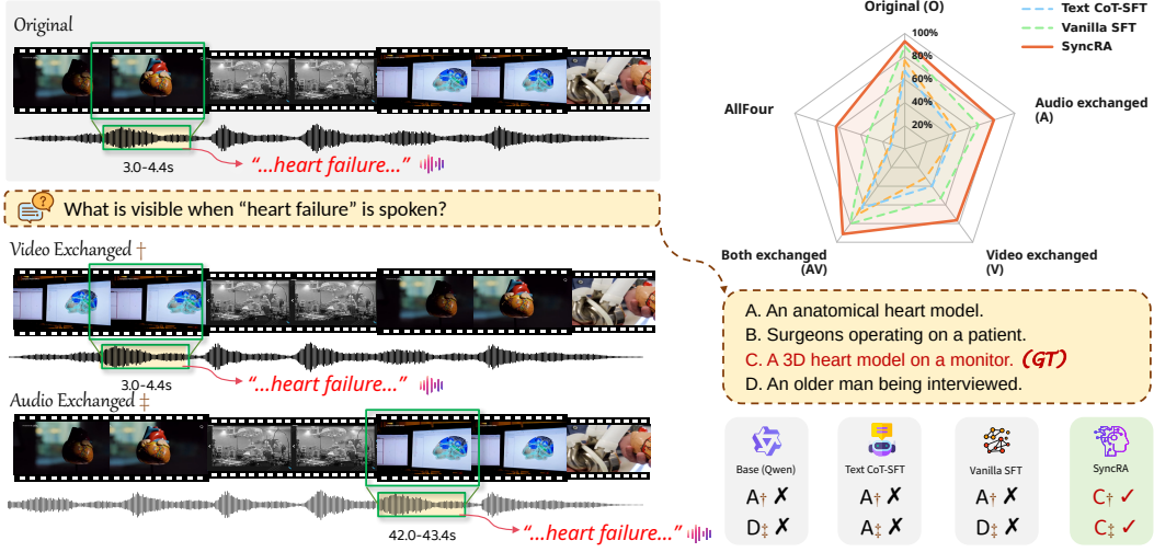
Figure 1: A motivating example and the swap diagnostic. Left: exchanging only the audio or only the video windows changes which scene is visible while “heart failure” is spoken (correct option A → C). Right: Qwen3-Omni accuracy on the four input versions (top; AllFour credits a cue only if all four are answered correctly) and predictions on the two illustrated exchanges (bottom; †/‡). SyncRA answers both correctly. Fine-tuned checkpoints use Run 1.
