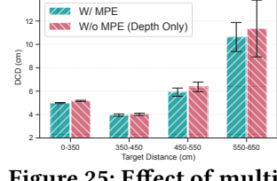
Figure 25: Effect of multi-primitive estimation (MPE) on point cloud reconstruction accuracy.
