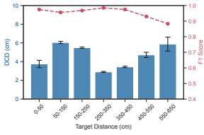
Figure 11: Overall performance.
