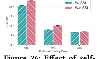
Figure 26: Effect of self-supervised pretraining with different amounts of labeled finetuning data.
