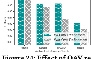
Figure 24: Effect of OAV refinement under different ambient thermal interferences.
