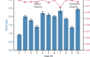
Figure 13: Cross-user performance.
