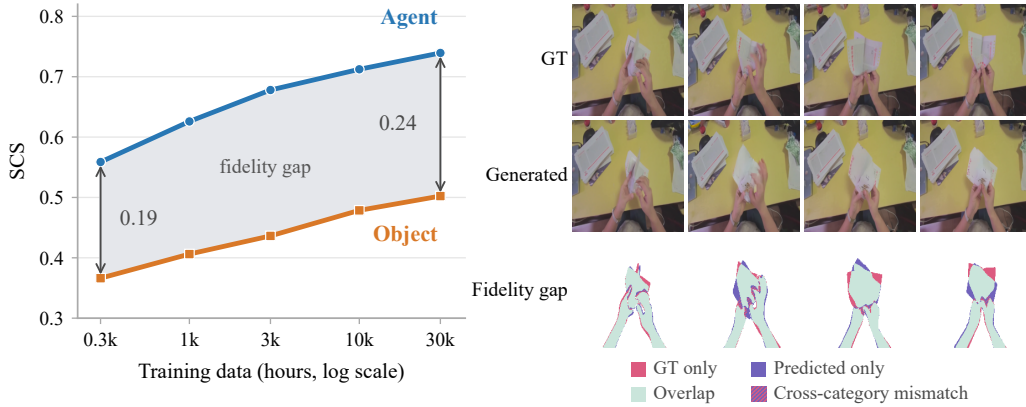
Figure 1: Limitations of world model scaling. Left: Ego-centric data scaling can achieve high agent modeling fidelity, but the effect of agent’s actions on the world lags behind. Right: The same failure at the level of a single prediction. Our best model places the hands almost exactly where they belong, while the paper they are folding is rendered in the wrong configuration throughout. See the project website for more video-level results.
