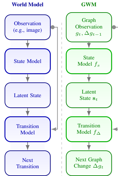
Figure 1: World Model (Ha & Schmidhuber, 2018) vs. Our Proposed GWM
