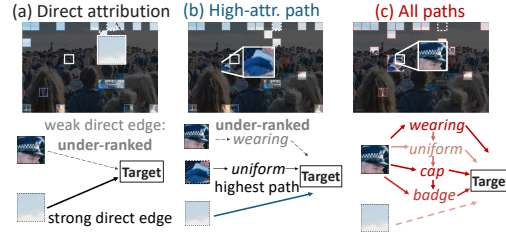
Figure 2: Tracing only highly-attributed paths misses evidence that many weaker paths carry.
