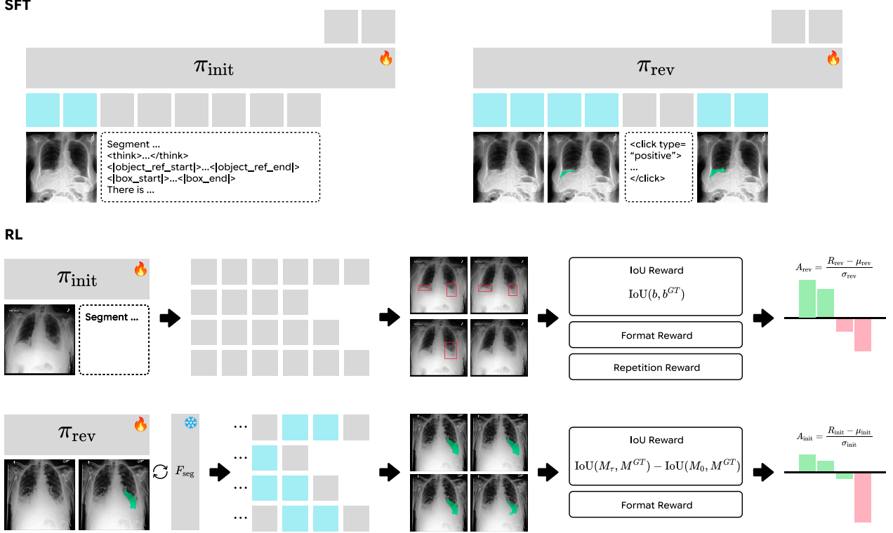
Figure 2: Training the two policies. We first apply SFT to \pi_{init} and \pi_{rev} on automatically constructed initial segmentation and segmentation revision scenarios, and then train each policy further with GRPO. A_{init} and A_{rev} are the advantages obtained by normalizing R_{init} and R_{rev} within each group of sampled generations. Text tokens are shown in gray and image tokens in light blue.
