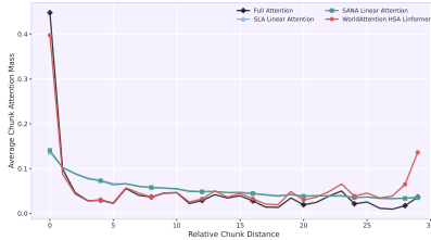
(a) Global attention mass.
