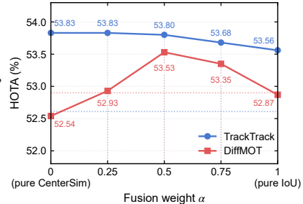
Figure 13: Fusion-weight sensitivity of TrackTrack and DiffMOT.
