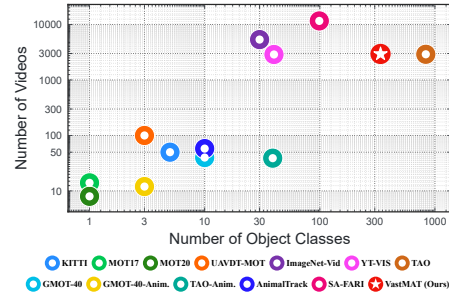
Figure 1: Category and video counts of VastMAT and representative tracking datasets.
