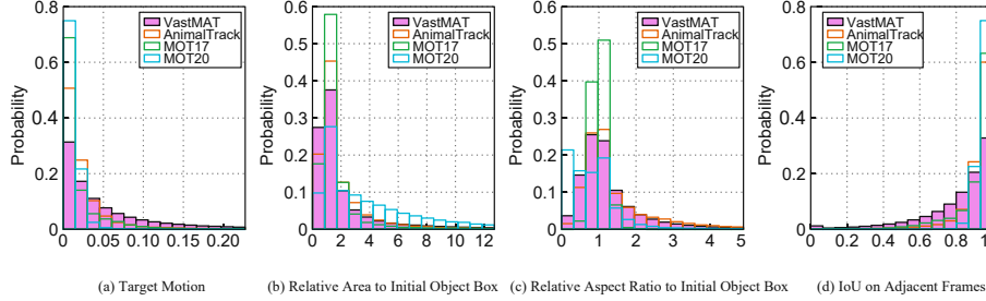
Figure 3: Motion and box-geometry distributions across tracking datasets.
