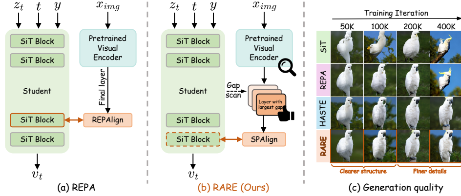
Figure 1: Alignment placed by convention and by measurement. (a) REPA alignment (REPA) pulls a fixed student block toward the teacher’s deepest layer for the whole run. (b) RARE first reads from a frozen checkpoint how much of each teacher layer the student still lacks, then applies sparse alignment (SPAlign): it aligns only the layer with the largest gap, puts more weight on tokens that are still far from the target, and switches the loss off once this distance stops falling, so alignment covers one layer and only the early part of training. (c) One class and noise draw at four training steps, guidance scale 4.0.
