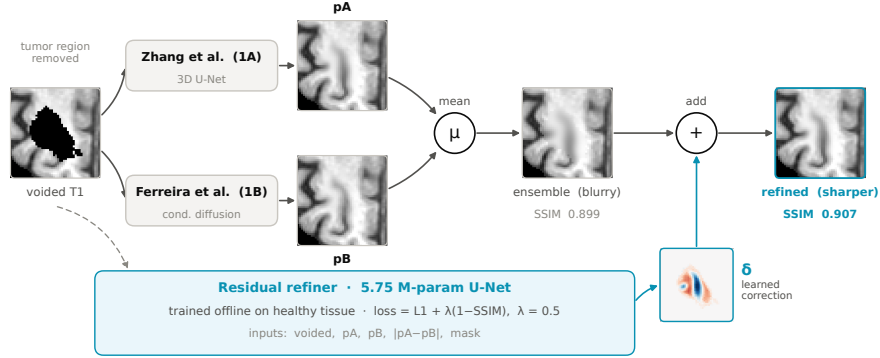
Fig. 1. Overview of the pipeline. The voided scan is passed to two frozen base models, the co-first-place entries of the 2025 challenge, 1A, Zhang et al. [25], and 1B, Ferreira et al. [8]. Their predictions p_A and p_B are averaged into the ensemble mean \bar{p} (Eq. 1), which is accurate but over-smoothed. The residual refiner, trained under Eq. 3 with \lambda = 0.5 , receives the voided scan, both predictions, their disagreement |p_A - p_B| and the void mask, and predicts a correction \delta added to \bar{p} (Eq. 2). Neither base model is fine-tuned. The blur of the “ensemble (blurry)” panel is exaggerated for display.
