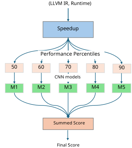
Figure 2: NCS intakes IRs and their corresponding runtimes. Each IR is tokenized, and each runtime is normalized to standardize the data. Next, the data is divided by performance percentiles (50-60%, 60-70%, ... , 90-100%), each of which is used to train a dedicated CNN model that classifies if the IR's performance will meet or exceed its target range. Finally, the predictions from each CNN model are summed to produce a comprehensive final score for ranking the configurations.
