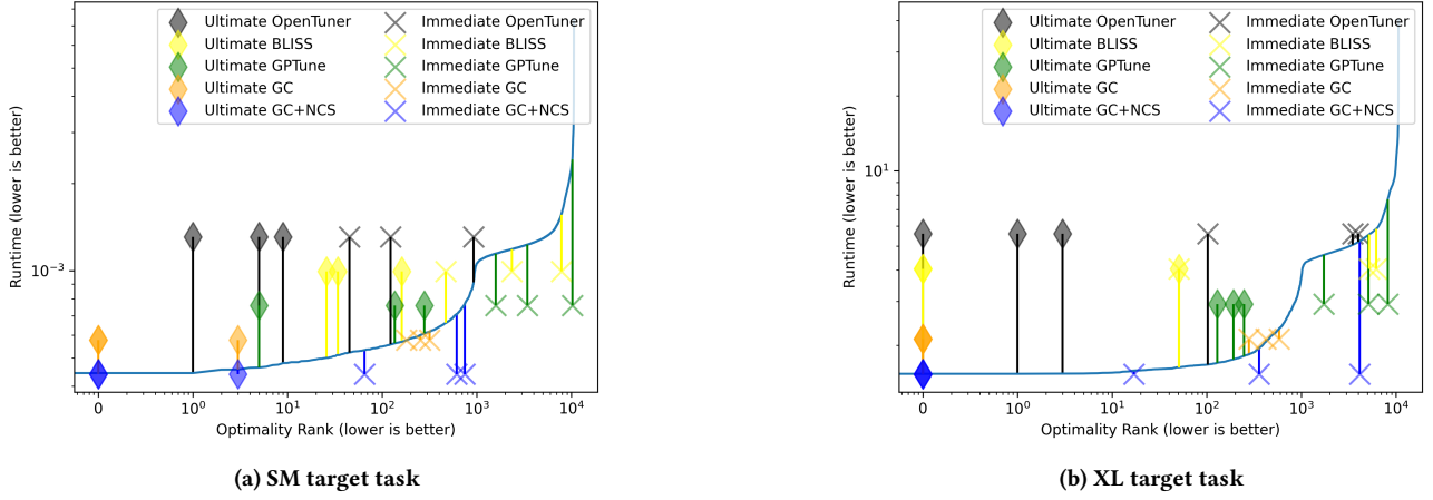
Figure 4: SyR2K overall search optimality per-seed shown on a log-log scale. Ideally, searches converge at the lowest rank.
