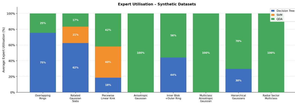
Figure 2: Average expert utilisation (%) on synthetic datasets for the proposed heterogeneous mixture model. Each stacked bar shows the proportion of samples assigned to the Decision Tree, SVM, and QDA experts by the gating mechanism, averaged over ten train-test splits.
