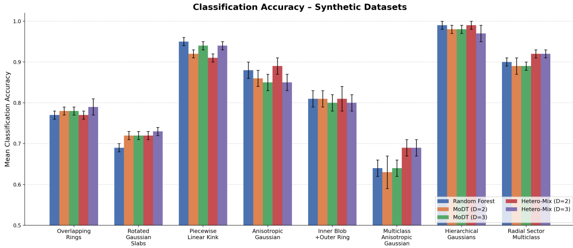
Figure 1: Mean classification accuracy on synthetic datasets. Error bars indicate one standard deviation over ten random train-test splits. Results are shown for Random Forest, MoDT (depth 2 and 3), and the proposed Hetero-Mix (depth 2 and 3).
