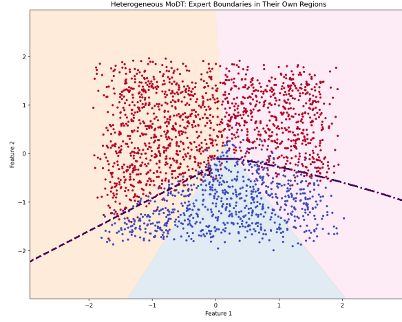
(c) Expert specialization learned by the heterogeneous Mixture Model.
