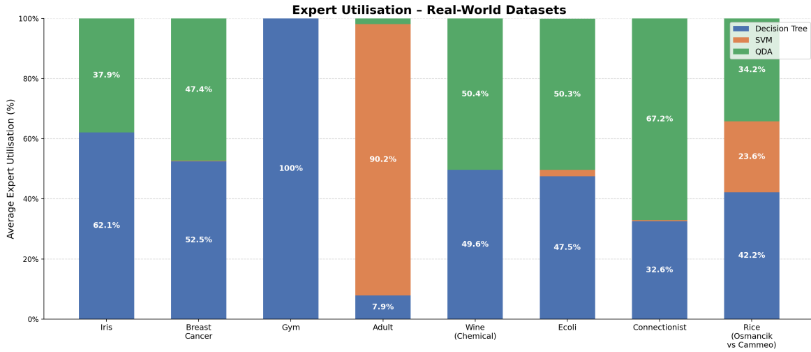
Figure 6: Average expert utilisation (%) on real-world datasets for the proposed heterogeneous mixture model. Each stacked bar shows the proportion of samples assigned to the Decision Tree, SVM, and QDA experts by the gating mechanism, averaged over ten train-test splits.
