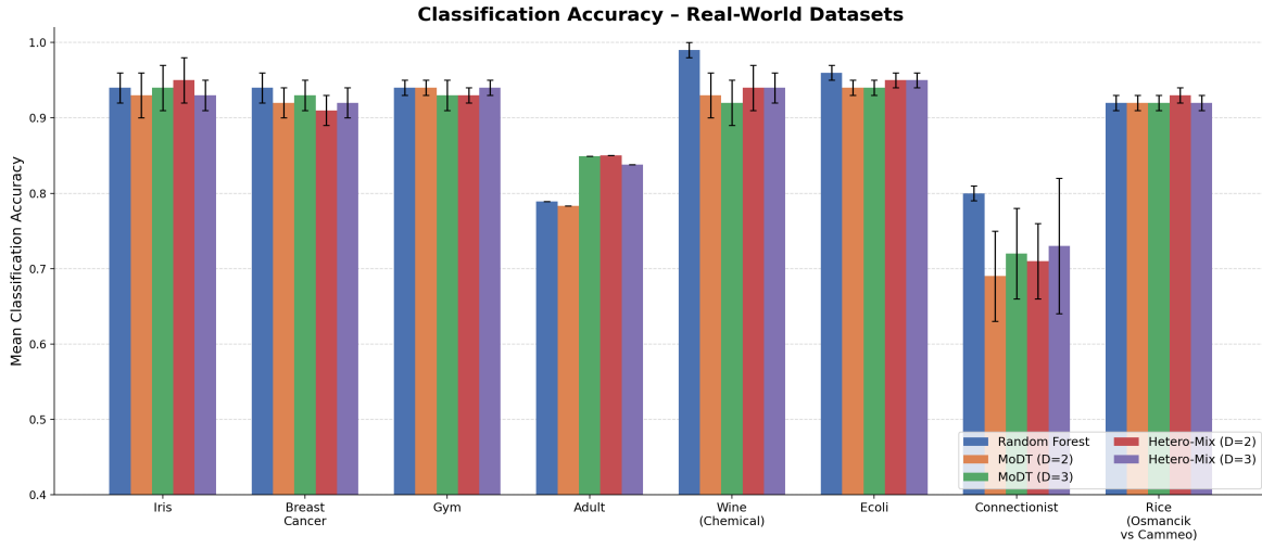
Figure 5: Mean classification accuracy on real-world datasets. Error bars indicate one standard deviation over ten random train-test splits. Results are shown for Random Forest, MoDT (depth 2 and 3), and the proposed Hetero-Mix (depth 2 and 3).
