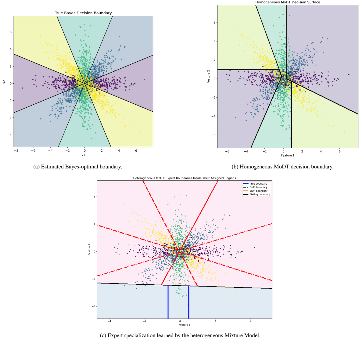
Figure 4: Comparison of decision boundaries and expert specialization on the Rotated Gaussian Slabs dataset. Subfigure (a) shows the estimated Bayes-optimal decision boundary obtained using quadratic discriminant analysis. Subfigure (b) presents the decision boundary learned by the MoDT composed exclusively of decision-tree experts. Subfigure (c) visualizes the specialization behavior learned by the proposed heterogeneous mixture framework. The shaded background denotes the dominant expert selected by the gating mechanism, where pink corresponds to the QDA expert, and blue corresponds to the decision-tree expert. Different colour of points denotes observations from different classes. Expert decision boundaries are displayed only within the regions where the corresponding expert receives dominant gating responsibility.
