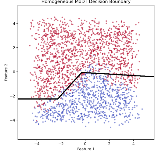
(b) Homogeneous MoDT decision boundary.
