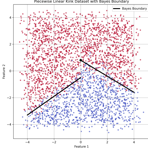
(a) Ground-truth decision boundary.
