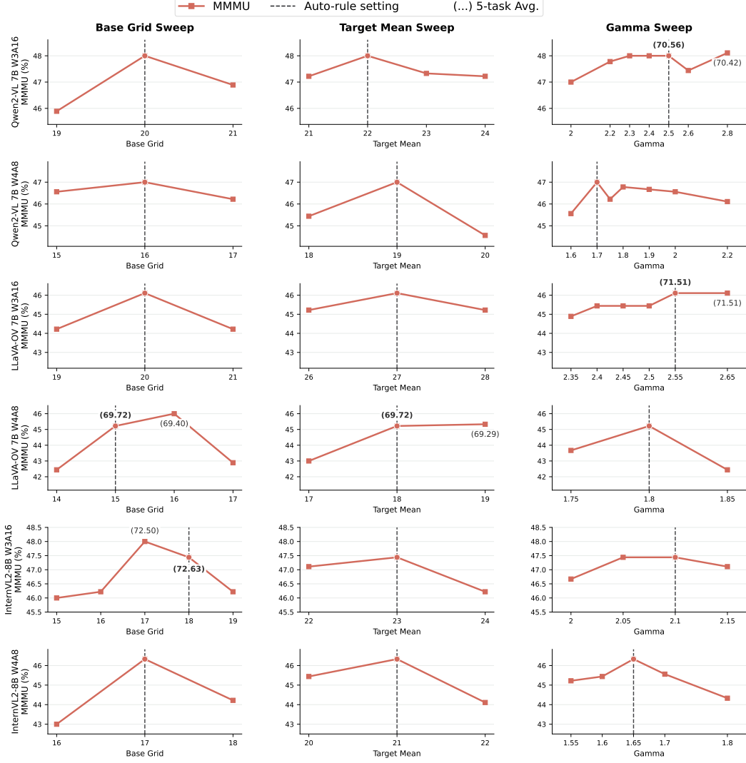
Figure 9: Analysis of the proposed Quantization Effect-Guided Allocation Rule. Each row corresponds to a model and setting, and each column sweeps one allocation dimension (base grid, target mean, or \gamma ) while keeping the others fixed. Numbers in parentheses indicate the 5-task average performance, and curves report MMMU performance. The dashed vertical line indicates the reference allocation in the sweep.
