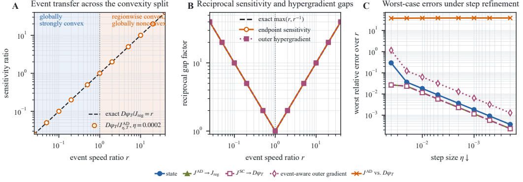
Figure 2: Convexity controls the residual-ReLU event transfer. (a) The endpoint-sensitivity ratio follows r across globally strongly convex attenuation, the C^1 interface, and nonconvex amplification, with fixed speed margin. (b) Endpoint- and outer-gradient reciprocal sensitivity ratios equal \max\{r, r^{-1}\} in the continuum limit. (c) State, regional-AD, and event-aware errors vanish under refinement, while ordinary AD remains separated from the flow derivative for r \neq 1 . Lines connect deterministic values.
