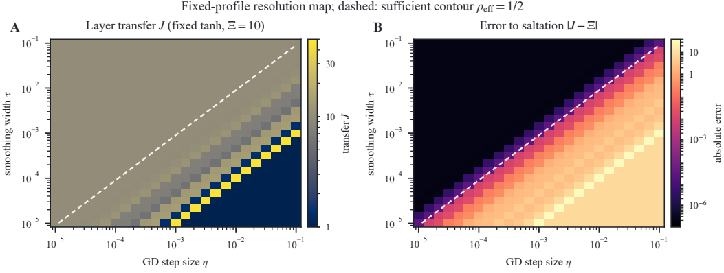
Figure 4: A fixed-profile smoothing resolution study. For the tanh profile and normalized window stated above, (a) shows the discrete tangent transfer and (b) its error to the saltation factor. The lightly marked contour is only the sufficient fixed-profile condition \rho_{\text{eff}} = 1/2 , not a necessary threshold. The theorem retains tail truncation and entry-phase dependence and makes no universality claim across smoothing families.
