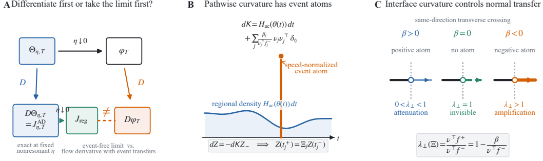
Figure 1: The discrete derivative limit omits atomic event curvature. (a) Fixed-step AD exactly differentiates each nonresonant GD program considered here; its limit is J_{\text{reg}} , while the flow derivative also contains event transfers. (b) Pathwise curvature consists of a regional density and speed-normalized event atoms. (c) Under same-direction transversality, positive, zero, and negative atomic curvature respectively attenuate, preserve, and amplify the direct normal mode.
