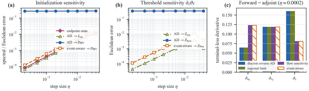
Figure 3: Matrix and parameter limits omit the same event. States approach the flow endpoints, while branchwise derivatives approach regional limits and remain separated from the flow derivatives; event-aware forward and adjoint calculations restore both.
