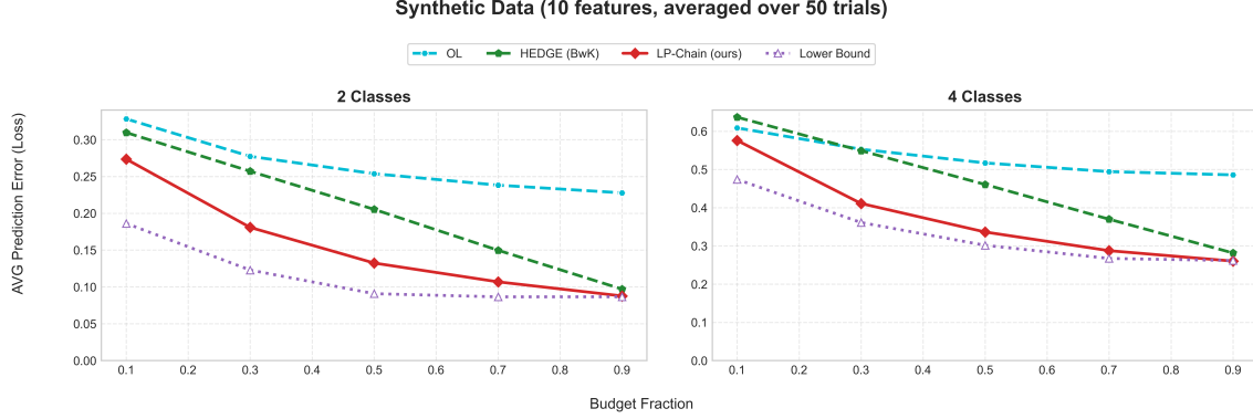
Fig. 1. Average prediction error versus budget fraction q on synthetic data. OL: Opportunistic Learning [9]; HEDGE (BwK): HEDGE-based BwK policy [12]; LP-Chain (ours): the proposed method; Lower Bound: prediction error of the full-action oracle \text{OPT}_{\text{LP}} . Lower is better.
