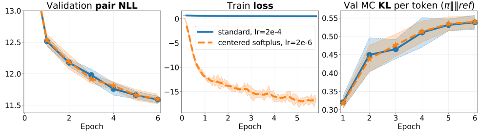
Figure I2: Comparison of training with the normalized centered-softplus DPO objective s_c(-\Delta; \beta) and standard DPO with pairwise loss -\log \sigma(\beta \Delta) on HelpSteer3 with Qwen3-4B-Instruct-2507 (batch size 24). SGD with \beta = 0.01 . The standard run uses \text{lr}_{\text{standard}} = 2 \times 10^{-4} and the centered-softplus run uses \text{lr}_{\text{norm}} = \beta \text{lr}_{\text{standard}} = 2 \times 10^{-6} . Curves show the mean over eight experiments; shaded bands denote one standard deviation.
