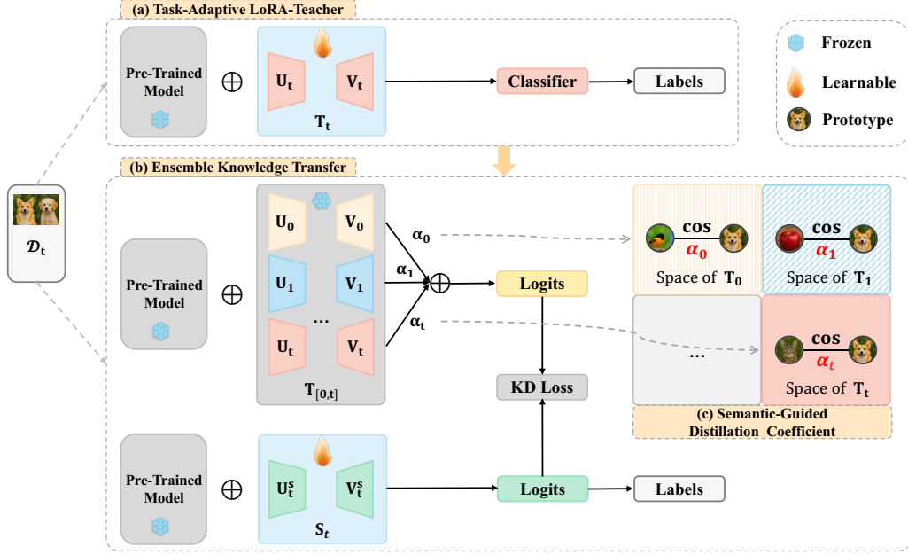
Figure 2: Overview of the TALON framework. (a) Task-Adaptive LoRA-Teacher: For each incremental task t , a new LoRA-Teacher T_t is trained to capture task-specific features while keeping previous LoRA-Teachers frozen. (b) Ensemble Knowledge Transfer: Multiple LoRA-Teachers are distilled into a unified LoRA-Student S_t using semantic-guided adaptive coefficients. (c) Semantic-Guided Distillation Coefficients \alpha_k : prototypes are extracted from the k -th LoRA-Teacher for task t data using Eq. (14), and the final coefficient \alpha_k is obtained by normalizing raw task-relevance scores in the shared feature space of LoRA-Teacher T_k according to Eq. (13).
