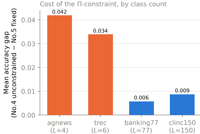
Figure 2: The accuracy cost of confining No.5 to the class-mean-orthogonal subspace (No.4 minus fixed No.5), averaged over k \in \{2, 3, 5, 10\} and three embedding sizes. The constraint costs almost nothing on the many-class datasets and a real, consistent amount on the few-class ones.
