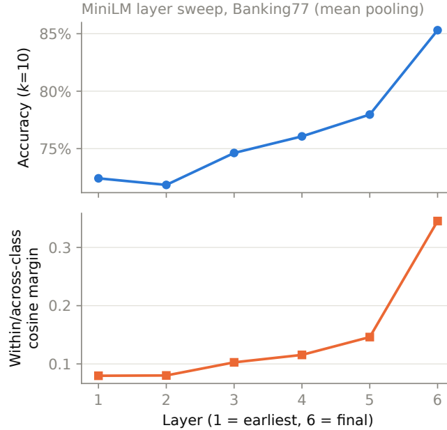
Figure 3: Layer sweep, MiniLM on Banking77. The within/across-class margin (bottom) tracks accuracy (top) almost exactly across layers of the same model, a predictive relationship that does not hold across different encoder architectures (Section 7).
