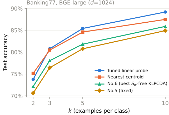
Figure 1: The headline comparison, Banking77 at d=1024 . The tuned linear probe and nearest centroid lead throughout; No.5, even after the tie-break fix (Section 3.3), remains a few points behind.
