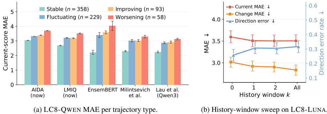
Figure 4: Fairness across trajectory types and the effect of dialogue history.
