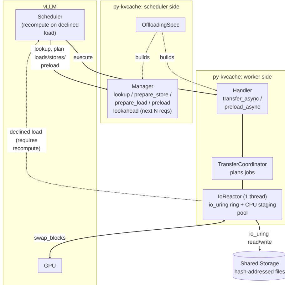
Figure 9: py-kvcache architecture.
