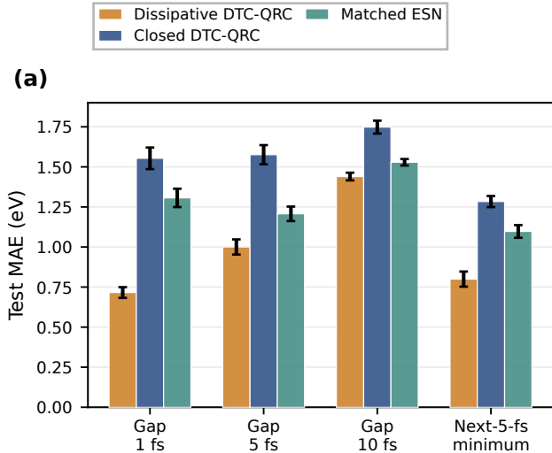
FIG. 3. Validation-selected SHNITSEL A01 application test at the common Q = 15 , T = 20 interface. Bars report test MAE for dissipative DTC-QRC, closed DTC-QRC, and the matched ESN using final-state Z + ZZ sampling and RBF-SVR. Error bars show six-seed sample standard deviations.
