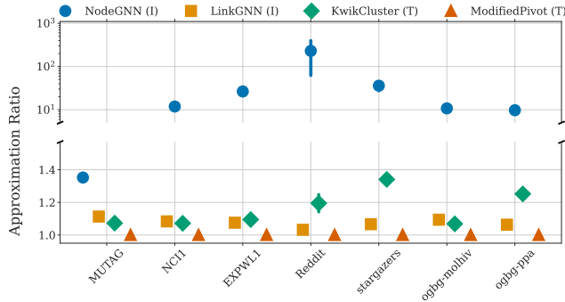
Figure 4: Comparison of methods in an inductive setting. Each point has error bars corresponding to the standard error of the mean, but are often too small. (I) was used to demark inductive methods, (T) for transductive ones. Values were normalized in each train/test split according to the minimum cost reached across methods.
