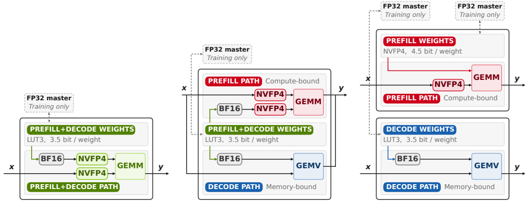
(a) Non-disaggregated quantized linear. Common model weights, same formats for the two phases. (b) Format-disaggregated quantized linear. Common model weights, phase-specific formats. (c) Fully-disaggregated quantized linear. Phase-specific model weights and formats.
