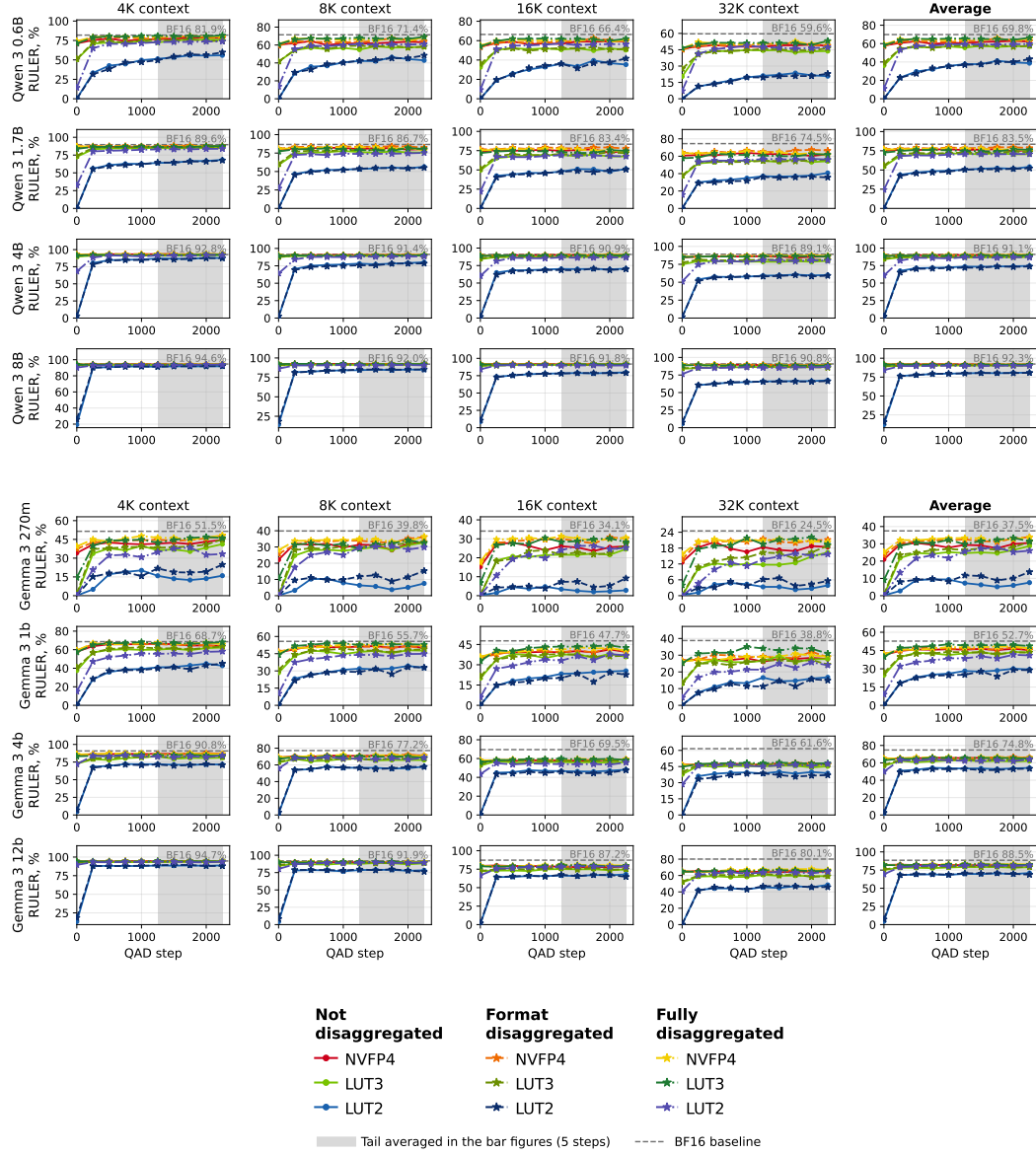
Figure 11: Breakdown of Figure 5 by context length and QADD step for prefill-heavy tasks.
