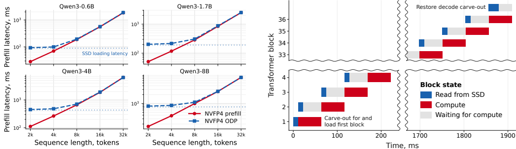
(a) NVFP4 prefill latency with and without ODP. Compute overtakes SSD loading at around 8K context and offloading overhead stays under 5% across Qwen 3 above 16K context.
