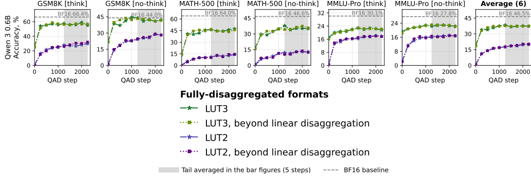
Figure 7: Fully-disaggregated quantization on Qwen3-0.6B with and without separation of the remaining unquantized parameters. This additional separation has no discernible effect on decode-heavy accuracy.
