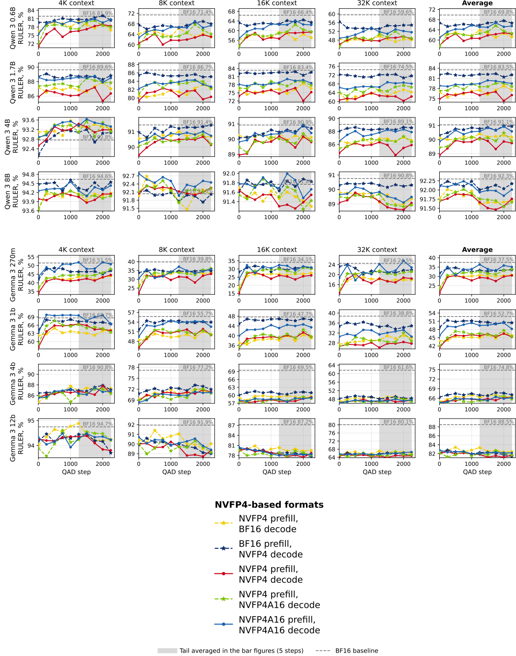
Figure 13: Breakdown of Figure 4 by context length and QADD step for prefill-heavy tasks.
