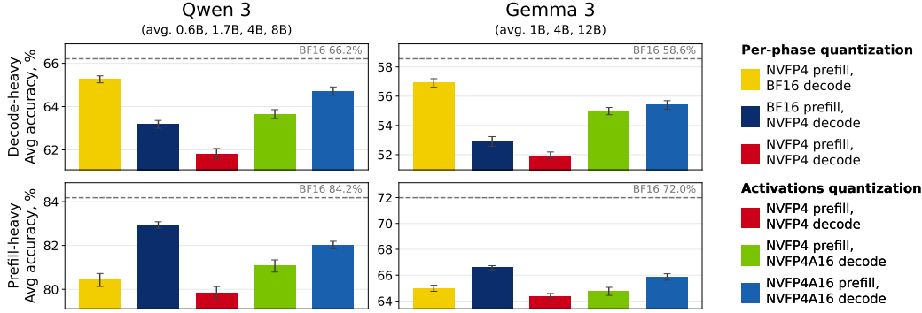
Figure 4: Family-mean accuracy of NVFP4-based formats after quantization-aware distillation on decode-heavy (top) and prefill-heavy (bottom) workloads. Decode-only NVFP4 quantization is more damaging than prefill-only quantization on decode-heavy tasks; the ordering reverses on prefill-heavy tasks. Format-disaggregated NVFP4 (green) combines NVFP4 prefill with NVFP4A16 decode and improves accuracy over uniform NVFP4 on both workloads without increasing weight storage or prefill cost. On decode-heavy tasks, it approaches the accuracy of NVFP4A16, which uses slower weight-only prefill.
