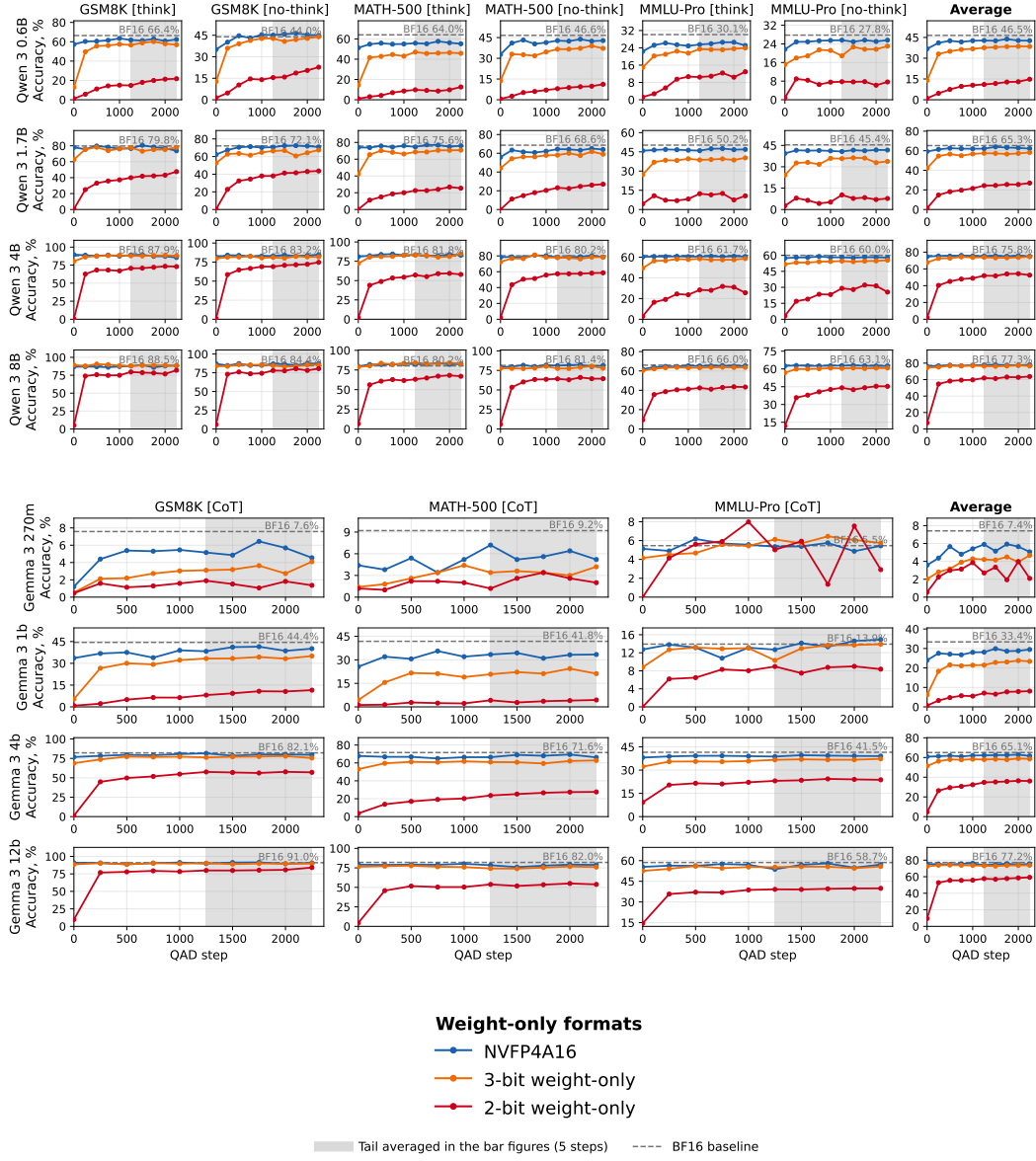
Figure 14: Performance breakdown for weight-only quantization formats by benchmark and QADD step.
