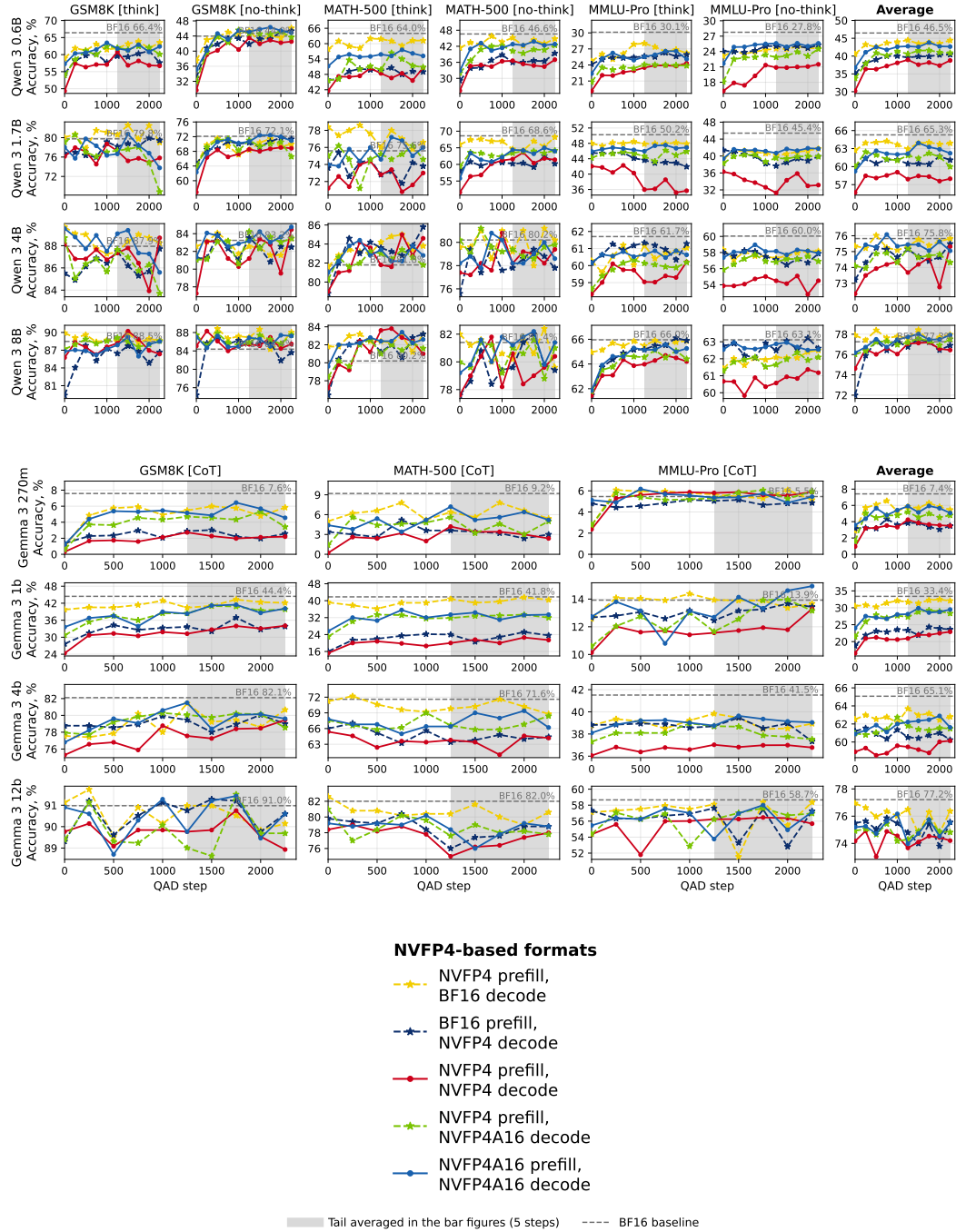
Figure 12: Breakdown of Figure 4 by benchmark and QADD step for decode-heavy tasks.
