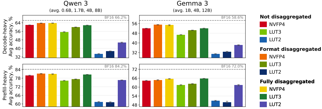
Figure 5: Family-mean accuracy of non-disaggregated, format-disaggregated and fully-disaggregated schemes with 2–4-bit decode weights and NVFP4 prefill compute after quantization-aware distillation. Format disaggregation primarily improves accuracy on decode-heavy tasks (top). Full disaggregation further improves low-bit accuracy on both workload types, with the largest gains over format disaggregation at 2-bit decode on prefill-heavy tasks.
