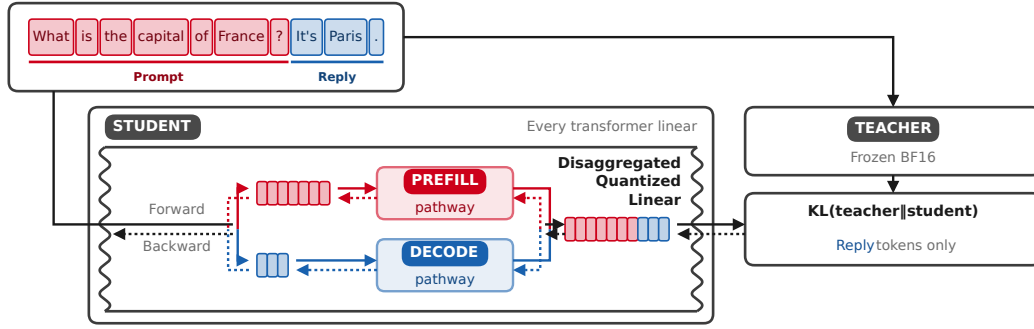
Figure 3: Quantization-aware distillation with disaggregation (QADD). The SFT assistant token mask, normally used only for loss, is also used to select the linear layer computational pathway.
