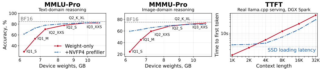
Figure 1: NVFP4 prefillers for off-the-shelf Qwen3.8-27B GGUF decoders. Left and middle: training the prefiller more than doubles IQ1_S accuracy on both benchmarks while leaving the decode checkpoint unchanged. ODP adds no weight-memory overhead. Right: measured time to first token in llama.cpp , comparing ODP with weight-only IQ1_S. ODP is faster from 4K context, reaching 1.78\times speedup at 8K.
