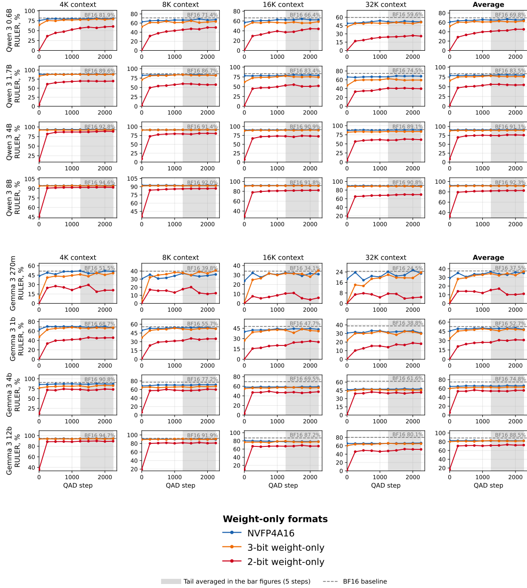
Figure 15: Performance breakdown for weight-only quantization formats on prefill-heavy tasks by context length and QADD step. The average excludes 64K evaluations.
