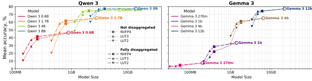
Figure 8: Decode-heavy accuracy of non-disaggregated and fully-disaggregated 2-4-bit quantized models with NVFP4 prefill versus encoded size of the quantized decode weights.
