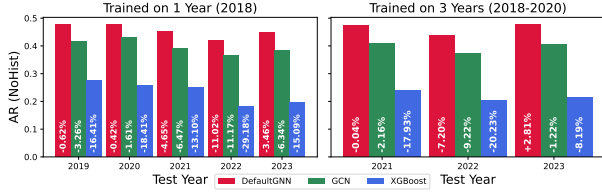
Figure 7: Comparison of model performances under OOT settings. Bar heights represent each model’s AR score on the NoHist subset, while values in the bars show how much the OOT performance of each model diverges from the original performance, i.e., training and testing on the same year.
