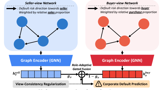
Figure 6: Overall framework of DefaultGNN. View-specific embeddings learned from multiplex transaction networks are fused via gating, regularized through view consistency. The fused embeddings are then used for default prediction.
